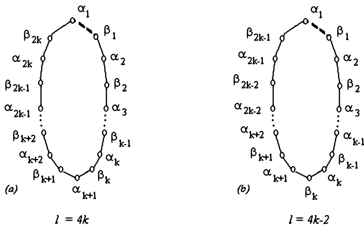
FIGURE 25. The two cases of even cycles D_l(b_{\frac{l}{2}-1}) : 1) l = 4k ; 2) l = 4k - 2
