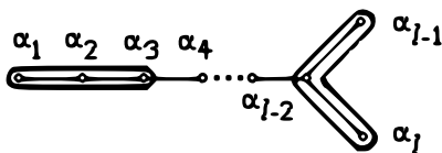
FIGURE 4. Elements s_{\alpha_1}s_{\alpha_3}s_{\alpha_2} and s_{\alpha_{l-1}}s_{\alpha_l}s_{\alpha_{l-2}} are not conjugate
