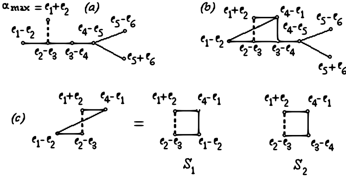
FIGURE 5. Equivalence of the C_1 -associated element w_1 and the C_2 -associated element w_2
