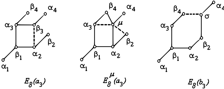
FIGURE 18. Equivalence E_8(b_3) \simeq E_8(a_3) ; E_8^\mu(a_3) is the connection diagram
