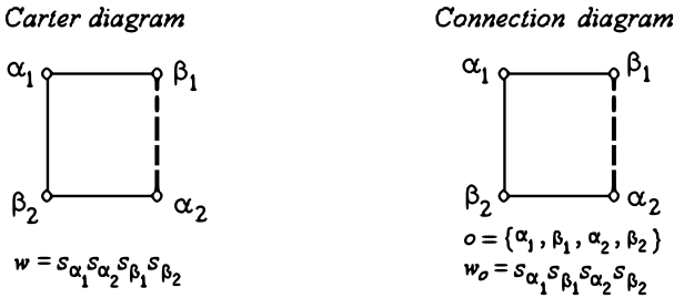
FIGURE 1. The Carter diagram D_4(a_1) and connection diagram (\mathcal{G}_4, o)
