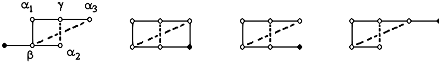
FIGURE 13. Not Carter diagrams on 6-vertices
