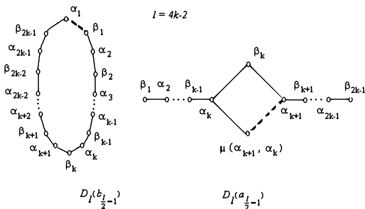
FIGURE 27. The equivalent diagrams D_l(b_{\frac{l}{2}-1}) and D_l(a_{\frac{l}{2}-1}) , where l = 4k - 2
