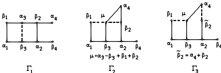
FIGURE 17. The equivalence transformation from \Gamma_1 to \Gamma_3
