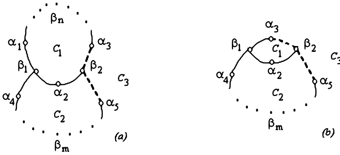
FIGURE 6. Intersecting cycles
