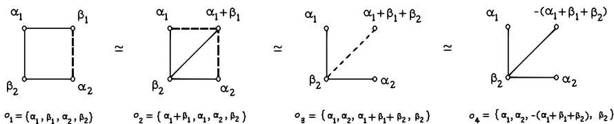
FIGURE 2. Eliminating of the cycle. The equivalence of (\mathcal{G}_4, o_1) and (D_4, o_4)
