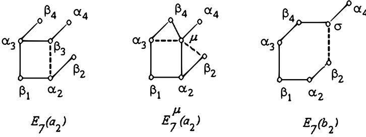
FIGURE 19. Equivalence E_7(b_2) \simeq E_7(a_2) ; E_7^\mu(a_2) is the connection diagram
