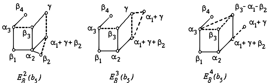
FIGURE 23. Step 3: E_8^2(b_5) \Rightarrow E_8^3(b_5) ; Step 4: E_8^3(b_5) \Rightarrow E_8^4(b_5) ; E_8^2(b_5) , E_8^3(b_5) , E_8^4(b_5) are connection diagrams
