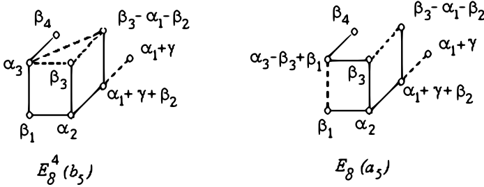
FIGURE 24. Step 5: E_8^4(b_5) \Rightarrow E_8(a_5) ; E_8^4(b_5) is the connection diagram
