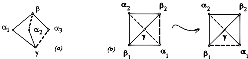
FIGURE 12. Every cycle should contain an odd number of dotted edges, a case which cannot happen
