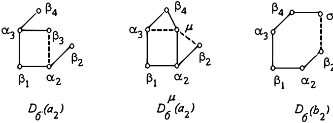
FIGURE 20. Equivalence D_6(b_2) \simeq D_6(a_2) ; D_6^\mu(a_2) is the connection diagram
