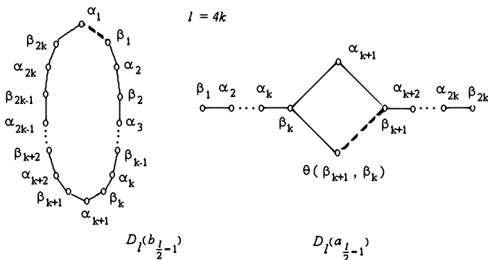
FIGURE 26. The equivalent diagrams D_l(b_{\frac{l}{2}-1}) and D_l(a_{\frac{l}{2}-1}) , where l = 4k
