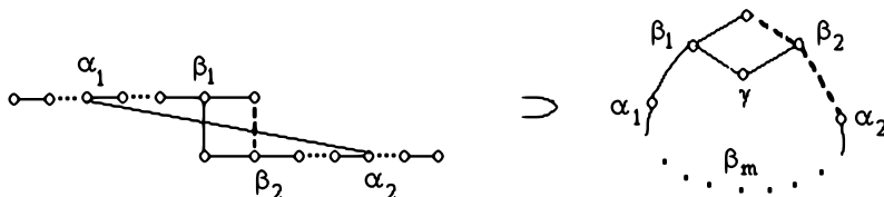
FIGURE 8. Two paths stemming from the opposite vertices of a 4-cycle
