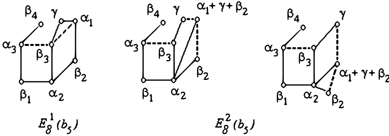
FIGURE 22. Step 2: E_8^1(b_5) \Rightarrow E_8^2(b_5) ; E_8^1(b_5) , E_8^2(b_5) are connection diagrams
