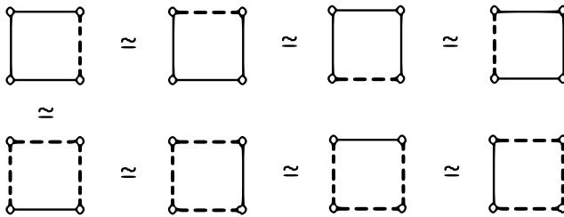
FIGURE 3. Eight similar 4-cycles equivalent to D_4(a_1)
