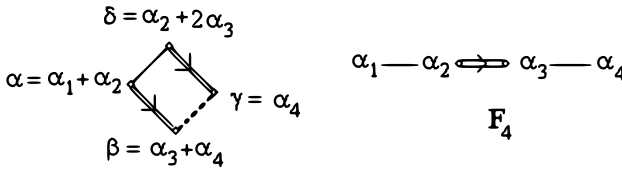
FIGURE 7. The 4-cycle root subset in F_4 . The angle (\widehat{\beta, \gamma}) is acute
