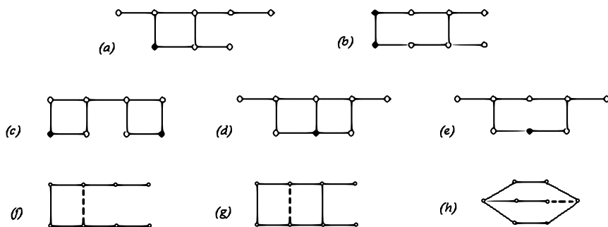
FIGURE 15. 8-vertex diagrams are not Carter diagrams
