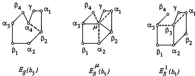
FIGURE 21. Step 1: E_8(b_5) \Rightarrow E_8^\mu(b_5) and E_8^\mu(b_5) \Rightarrow E_8^1(b_5) ; E_8^\mu(b_5) , E_8^1(b_5) are connection diagrams
