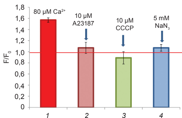
Fig. 8. Effects of \text{Ca}^{2+} -ionophore and mitochondria-deenergizing compounds on matrix \text{Ca}^{2+} content (the cation had been accumulated in energy-dependent manner); F_0 – Fluo-4 AM fluorescent signal without exogenous \text{Ca}^{2+} addition (endogenous ionized Ca, ‘starting’ level), F – Fluo-4 AM fluorescent signal with addition of exogenous \text{Ca}^{2+} and the investigated compounds, ( M \pm m , n = 5 ). Flow cytometry data
