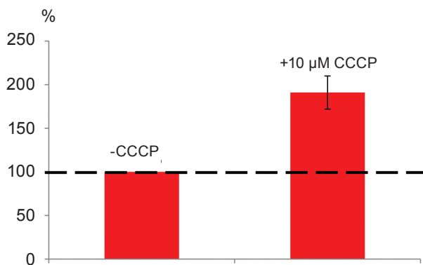
Fig. 7. Increase in myoplasm \text{Ca}^{2+} concentration in intact cells under the effect of CCCP protonophore (control values are taken as 100%); M \pm m , 8 cells from independent experiments were used for the analysis. Fluo-4 AM fluorescence in cells without the effectors is taken as 100% (ordinate axis). Confocal microscopy data
