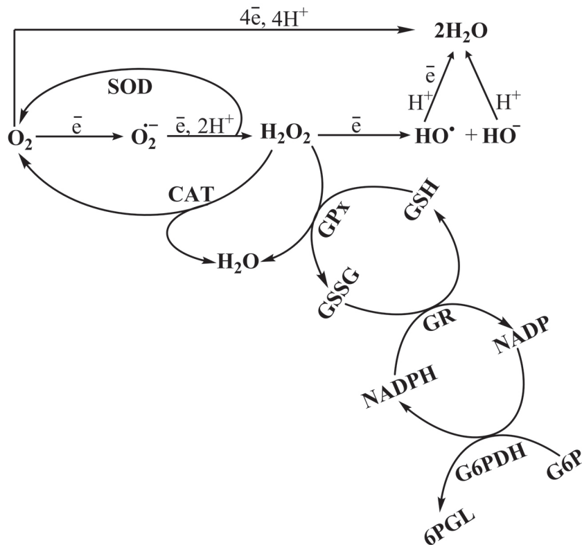
Fig. 1. Four- and consistent one-electron reduction of molecular oxygen and antioxidant enzymes of the first and second lines. Addition of one electron to oxygen molecule leads to the formation of superoxide anion radical ( O_2^{\cdot-} ). Further addition of one more electron to O_2^{\cdot-} leads to the formation of hydrogen peroxide ( H_2O_2 ), which is not a radical. One-electron H_2O_2 reduction leads to the formation of the hydroxyl radical ( HO^{\cdot} ) and hydroxyl anion. Finally, addition of one more electron and proton to HO^{\cdot} results in water molecule formation. Two above-mentioned partially reduced oxygen species, namely O_2^{\cdot-} and HO^{\cdot} are free radicals, but H_2O_2 is not. All together forms of partially reduced oxygen ( O_2^{\cdot-} , H_2O_2 , and HO^{\cdot} ) have higher chemical reactivity than molecular oxygen, due to which they were collectively named as "reactive oxygen species" (ROS). Transformation of O_2^{\cdot-} to H_2O_2 is significantly accelerated by certain enzymes, called primary antioxidant enzymes. The first enzyme in this chain is called superoxide dismutase (SOD) and it catalyzes a redox reaction of disproportionation of two O_2^{\cdot-} molecules resulting in formation of molecular oxygen and hydrogen peroxide. The next component in the chain of one-electron O_2 reduction of ROS, H_2O_2 may be converted to less harmful species by several enzymes of a large group called peroxidases. Catalase dismutates H_2O_2 to molecular oxygen and water, while glutathione dependent peroxidases (GPx) using glutathione as a cofactor reduce it to water. Since currently there is no reliable information on the existence of specific enzyme systems dealing with hydroxyl radicals, it is generally accepted that prevention of its formation is the best way to combat it. Abbreviations: CAT – catalase; GPx – glutathione dependent peroxidase; GR – glutathione reductase; G6PDH – glucose-6-phosphate dehydrogenase; G6P – glucose-6-phosphate; 6PGL – 6-phosphogluconate; GSH and GSSG – reduced and oxidized forms of glutathione; NADP and NADPH – oxidized and reduced forms of nicotinamide adenine dinucleotide phosphate; SOD – superoxide dismutase
