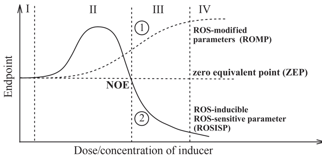
Fig. 3. Schematic presentation of the intensity-based classification of oxidative stresses. Curve 1 indicates the level of ROS-modified cell component/parameter (ROMP), whereas curve 2 shows ROS-inducible ROS-sensitive parameter (ROSISP), such as activity of antioxidant enzyme or cell survival. In fact, the curves 1 and 2 show the relationship between the dose/concentration of the oxidative stress inducer and the parameters typically used to characterize the stress and which can be experimentally measured. Zone I – basal oxidative stress (BOS), where there is no observable effects that cannot be registered due to the very low intensity of oxidative stress; Zone II – low intensity oxidative stress (LOS) with slightly increased level of ROS-modified molecules and enhanced activity of antioxidant enzymes or cell survival in response to enhanced ROS level; Zone III – strong oxidative stress (SOS); and Zone IV – very strong oxidative stress (VOS), where the values of the recorded parameters reach nearly maximum/minimum values. Abbreviations: NOE – no observable effect point; ZEP – zero equivalent point – the level of components of interest corresponds to the initial (basic) level in the absence of inducer of oxidative stress. (Modified from [18, 19])
