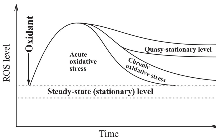
Fig. 2. Schematic presentation of the time-course based classification of oxidative stresses. Usually, the stationary ROS concentration is maintained within a certain range and oscillates like other parameters in the body according to homeostasis theory. However, under certain circumstances, ROS concentration may leave this corridor due to increased generation or decreased elimination. Conditions when ROS level is increased for a short time period with certain functional consequences has been called “acute oxidative stress”, while a prolonged increase in ROS levels accompanied by such consequences is called “chronic oxidative stress”. In some cases, the level of ROS is not returned into the original corridor or close to it and may stabilize at a higher steady-state level, called quasi-stationary one. Both acute and chronic oxidative stresses may have different effects on living organisms and cause more or less significant damage to the cells and, if the system is unable to regain control, it can lead to cell death from apoptosis or necrosis
