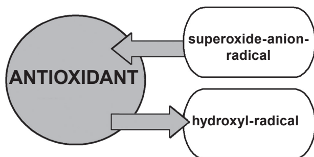
Fig. 4. Scheme of redistribution of electron density under interaction of MLT and GSH molecules with \bullet\text{OH} and \bullet\text{OO}^-
