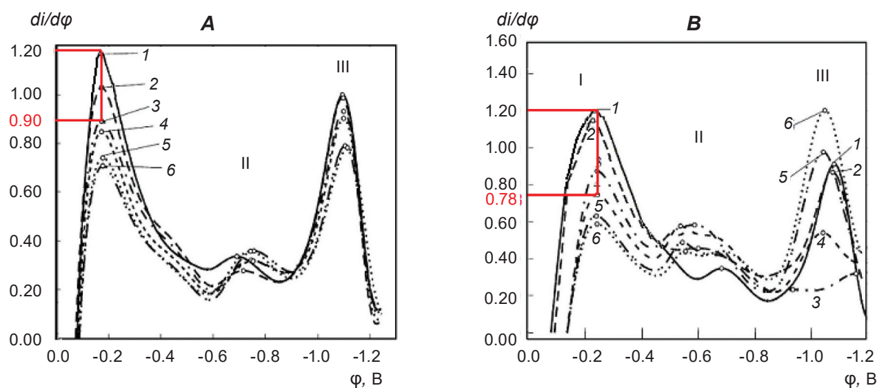
Fig. 5. Differential voltamperograms of FR reduction on a copper cathode on the background of 0.1M NaCl in water (I) in the presence of various concentrations of antioxidants: MLT (A): 2 – 0.39; 3 – 0.74; 4 – 1.07; 5 – 1.67; 6 – 2.18 \cdot 10^{-3} \text{ M/dm}^3 ; GSH (B): 2 – 0.24; 3 – 0.47; 4 – 0.74; 5 – 0.91; 6 – 1.1 \cdot 10^{-3} \text{ M/dm}^3
