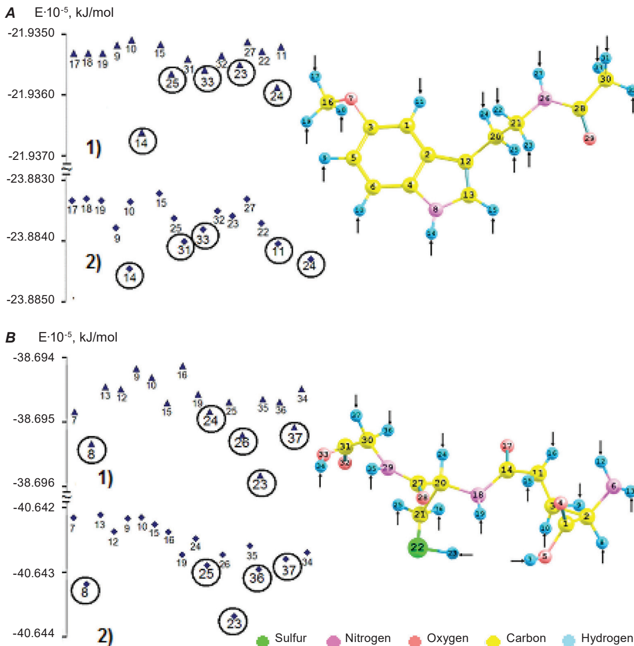
Fig. 1. Minimums of full interaction energy ( E ) in complexes: A – MLT \cdots OH[ \cdot OO^- ] ; B – GSH \cdots OH[ \cdot OO^- ] under the “attack” of various centers of antioxidant molecules by free radicals: 1 – \cdot OH ; 2 – \cdot OO^- (5 the deepest minimums – O are distinguished)
