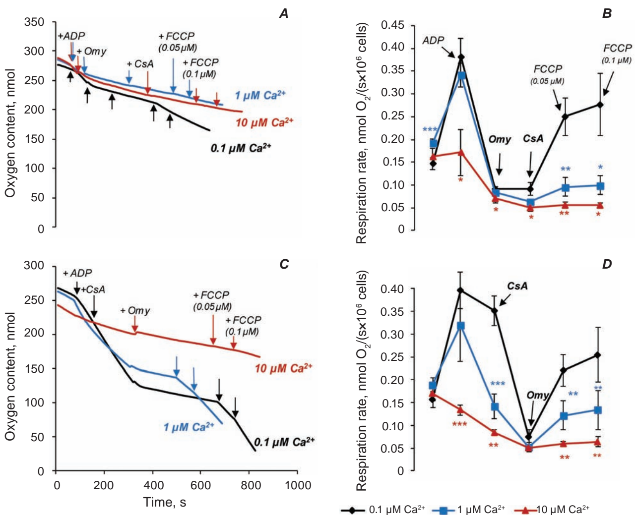
Fig. 2. Effect of CsA on the permeabilized hepatocytes respiration rate at oxidation of malate, glutamate and pyruvate mixture in media with 0.1, 1 and 10 \mu\text{M} \text{Ca}^{2+} : original record of oxygen consumption by the hepatocytes suspension at successive addition of Omy – CsA (A) or CsA – Omy (C) into the chamber; hepatocytes respiration rate at successive addition of Omy – CsA (B) or CsA – Omy (D) into the chamber; [malate] = 5 mM, [glutamate] = 5 mM, [pyruvate] = 5 mM, [ADP] = 750 \mu\text{M} , [CsA] = 0.5 \mu\text{M} , [Omy] = 3 \mu\text{M} , [FCCP] = 0.05 and 0.1 \mu\text{M} ; via asterisk the statistically significant difference was denoted just compared to 0.1 \mu\text{M} \text{Ca}^{2+} with * P < 0.05 , ** P < 0.01 or *** P < 0.001 ; n = 7
