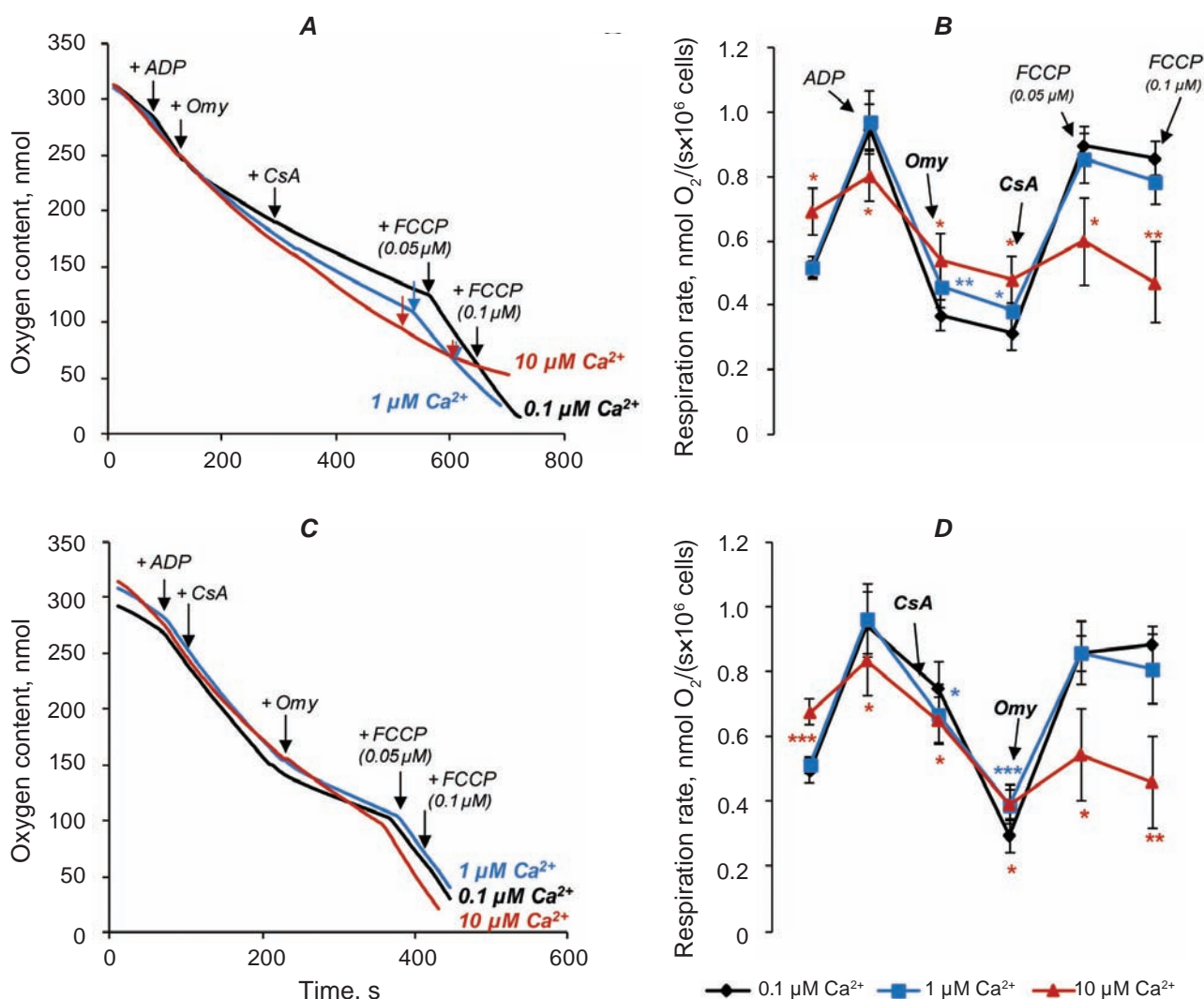
Fig. 1. Effect of CsA on the permeabilized hepatocytes respiration rate at succinate oxidation in media with 0.1, 1 and 10 \mu\text{M} \text{Ca}^{2+} : original record of oxygen consumption by the hepatocytes suspension at successive addition of Omy – CsA (A) or CsA – Omy (C) into the chamber; hepatocytes respiration rate at successive addition of Omy – CsA (B) or CsA – Omy (D) into the chamber; [succinate] = 5 mM, [ADP] = 750 \mu\text{M} , [CsA] = 0.5 \mu\text{M} , [Omy] = 3 \mu\text{M} , [FCCP] = 0.05 and 0.1 \mu\text{M} ; via asterisk the statistically significant difference was denoted just compared to 0.1 \mu\text{M} \text{Ca}^{2+} with * P < 0.05 , ** P < 0.01 or *** P < 0.001 ; n = 7
