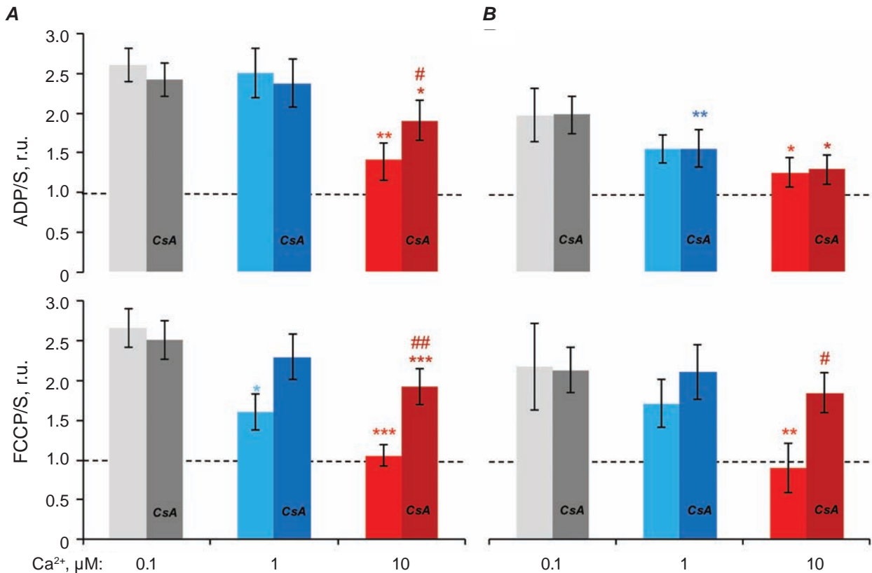
Fig. 6. Respiratory control of permeabilized hepatocytes in the medium containing 0.1, 1 and 10 \mu\text{M} \text{Ca}^{2+} in the absence or presence of CsA: A – at succinate oxidation; B – at mixture of malate, glutamate and pyruvate oxidation; [succinate] = 5 mM, [malate] = 5 mM, [glutamate] = 5 mM, [pyruvate] = 5 mM, [CsA] = 0.5 \mu\text{M} , [ADP] = 750 \mu\text{M} , [FCCP] = 0.25 \mu\text{M} ; *statistically significant difference compared to 0.1 \mu\text{M} \text{Ca}^{2+} ; #statistically significant difference compared to control (without CsA); n = 7
