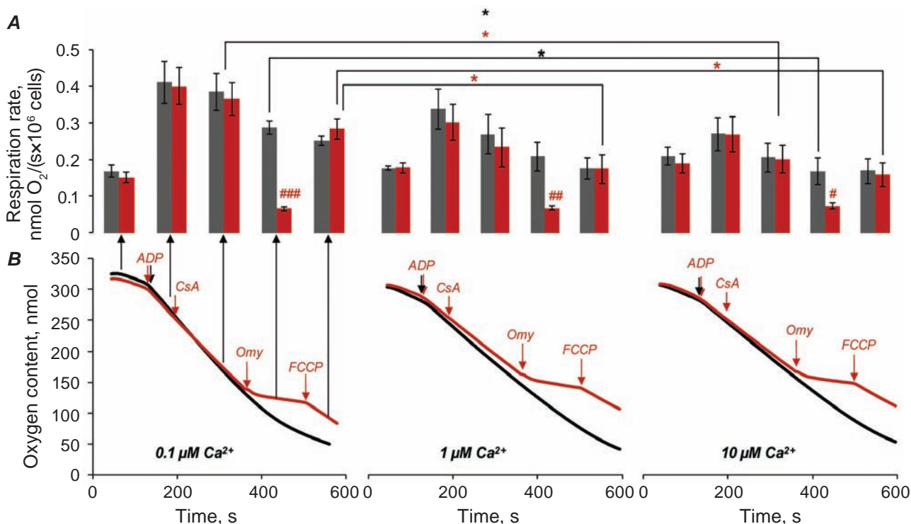
Fig. 3. Hepatocytes respiration is reduced not due to CsA influence: permeabilized hepatocytes respiration rate (A) and original record of oxygen consumption (B) at oxidation of malate, glutamate and pyruvate mixture; [malate] = 5 mM, [glutamate] = 5 mM, [pyruvate] = 5 mM, [ADP] = 750 \mu\text{M} , [CsA] = 0.5 \mu\text{M} , [Omy] = 3 \mu\text{M} , [FCCP] = 0.05 \mu\text{M} ; *statistically significant difference compared to 0.1 \mu\text{M} \text{Ca}^{2+} ; #statistically significant difference compared to control (without CsA); n = 6
