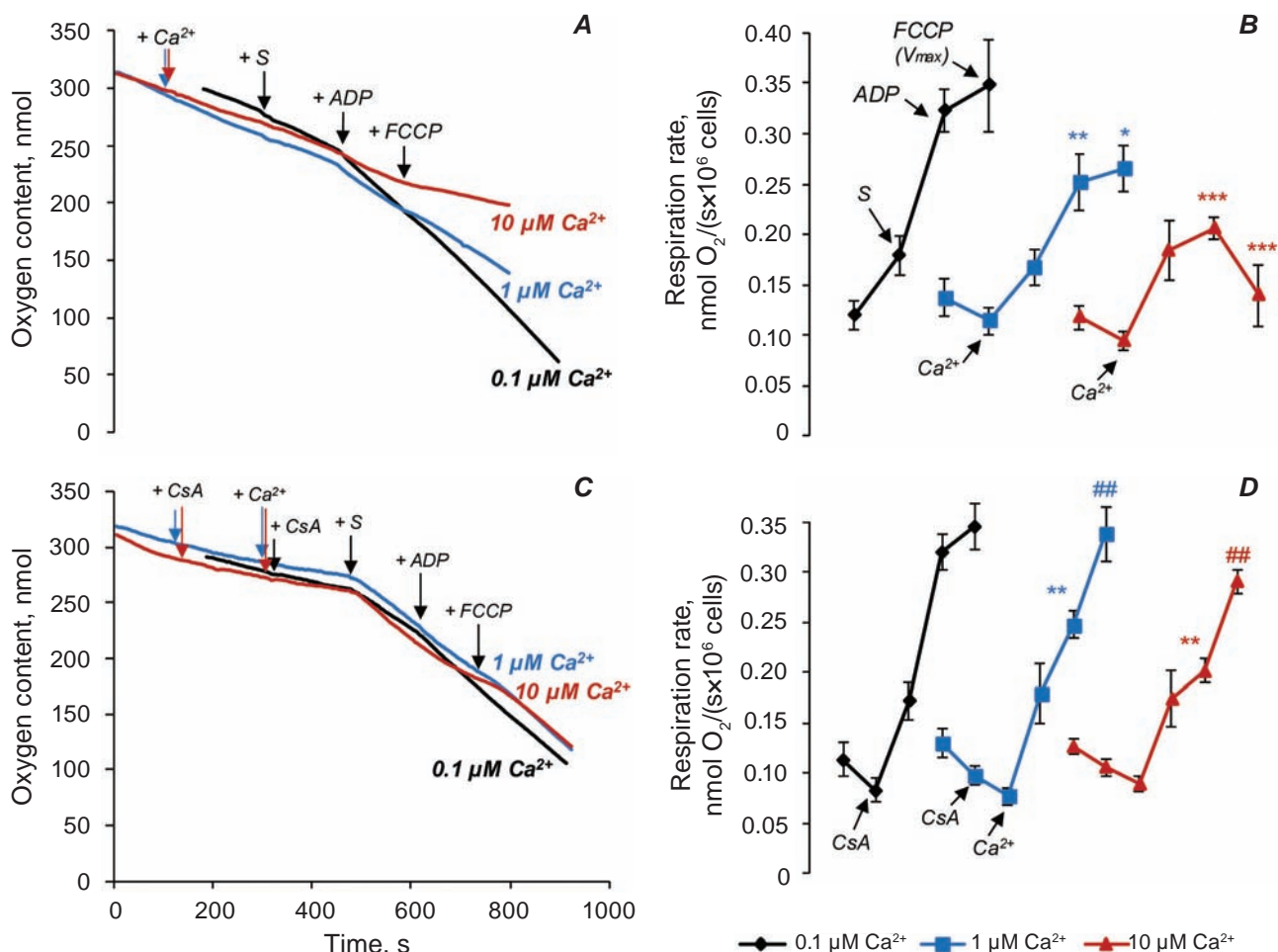
Fig. 5. Effect of CsA on oxygen consumption rate by permeabilized hepatocytes at mixture of malate, glutamate and pyruvate oxidation in the mediums with 0.1, 1 and 10 \mu\text{M Ca}^{2+} : original record of oxygen consumption by the hepatocytes suspension at CsA absence (A) and CsA presence (C) within the medium; hepatocytes respiration at CsA absence (B) and CsA presence (D) within the medium; [malate] = 5 mM, [glutamate] = 5 mM, [pyruvate] = 5 mM, [CsA] = 0.5 \mu\text{M} , [ADP] = 750 \mu\text{M} , [FCCCP] = 0.25 \mu\text{M} ; *statistically significant difference compared to 0.1 \mu\text{M Ca}^{2+} ; #statistically significant difference compared to control (without CsA); n = 7
