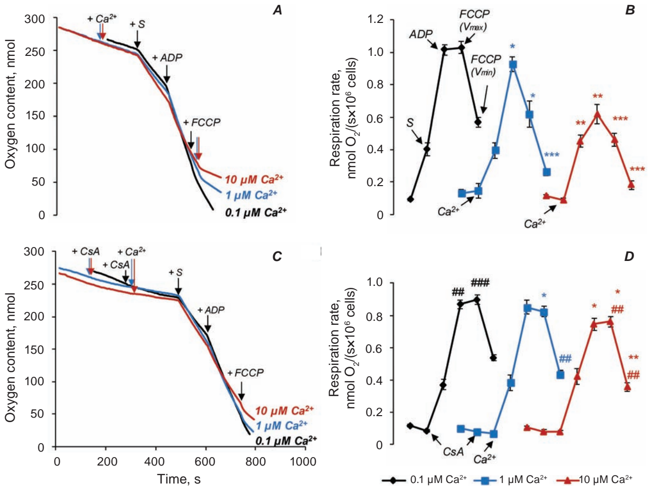
Fig. 4. Effect of CsA on oxygen consumption rate by permeabilized hepatocytes at the succinate oxidation in the mediums with 0.1, 1 and 10 \mu\text{M} \text{Ca}^{2+} : original record of oxygen consumption by the hepatocytes suspension at CsA absence (A) and CsA presence (C) within the medium; hepatocytes respiration at CsA absence (B) and CsA presence (D) within the medium; [succinate] = 5 mM, [CsA] = 0.5 \mu\text{M} , [ADP] = 750 \mu\text{M} , [FCCP] = 0.25 \mu\text{M} ; *statistically significant difference compared to 0.1 \mu\text{M} \text{Ca}^{2+} ; #statistically significant difference compared to control (without CsA); n = 6
