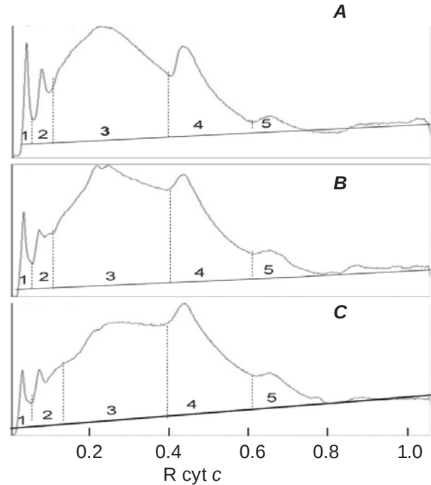
Fig. 3. Electrophoretic plots of three types of “Chitopharm” chitosan samples. A – “Chitopharm”L (lane 1 in Fig. 2, A); B – “Chitopharm”M (lane 2 in Fig. 2, A); C – “Chitopharm”S (lane 3 in Fig. 2, A). Dashed lines mark limits of peaks in quantitative analysis
