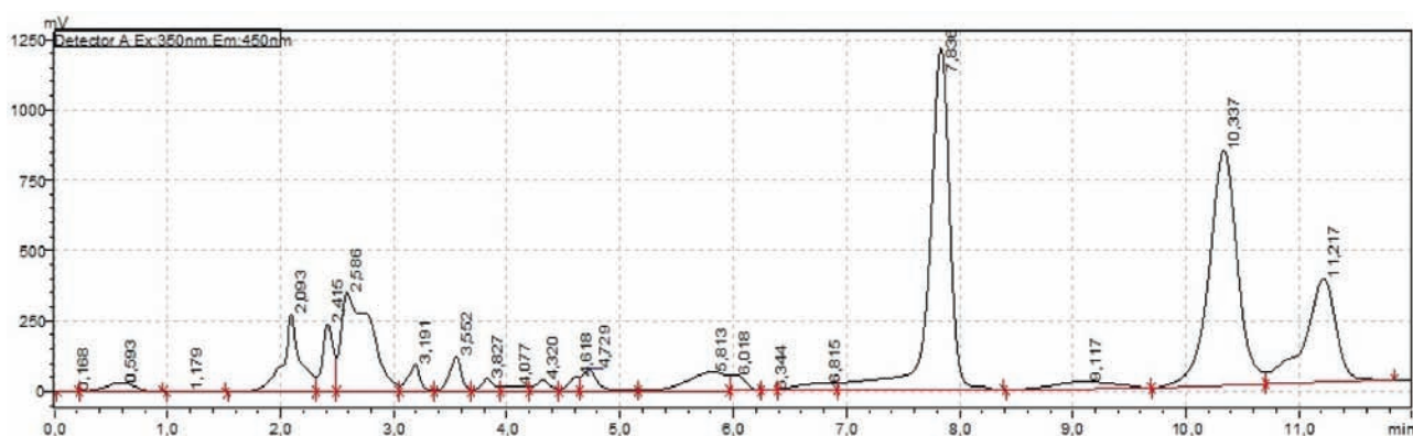
Fig. 1. Agmatine peaks. A – The peak with a retention time of 7.741 min was the derivative reagent, and 10.124 min was the standard agmatine peak. B – The peak with a retention time of 7.838 min was the derivative reagent, and 10.337 min was the plasma agmatine peak
