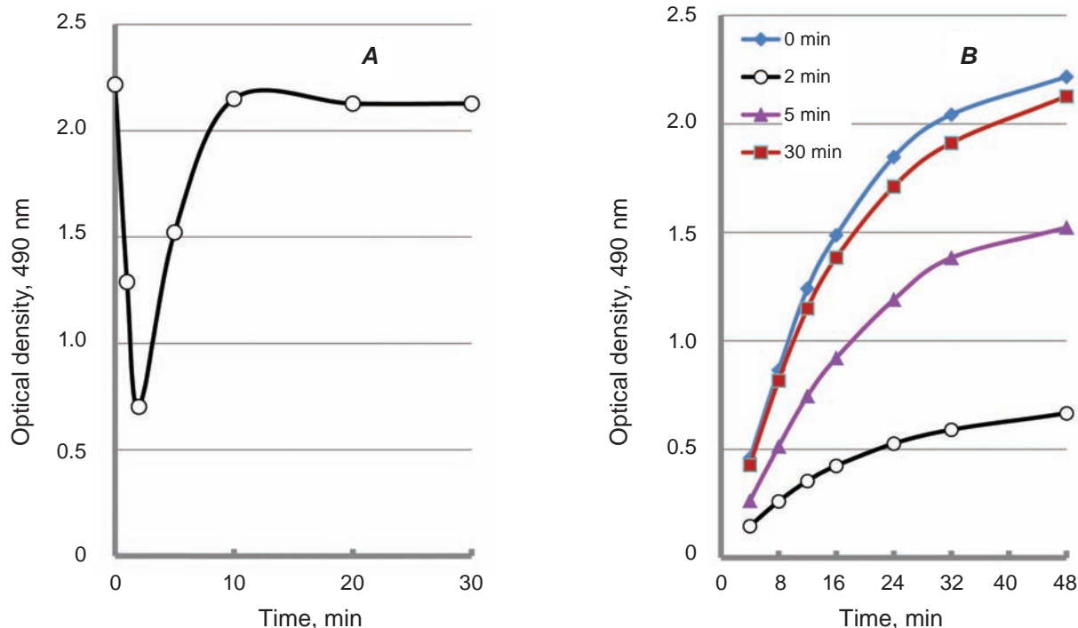
Fig. 5. A – Effect of incubation time of mAbs in 25% TFE at 0°C on mAbs reactivity against ovalbumin; B – Dynamic of the binding of mAbs to antigen immobilized on plate for control (0 min) mAbs or mAbs pre-treated during 2 min, 5 min or 30 min with 25% TFE at 0°C
