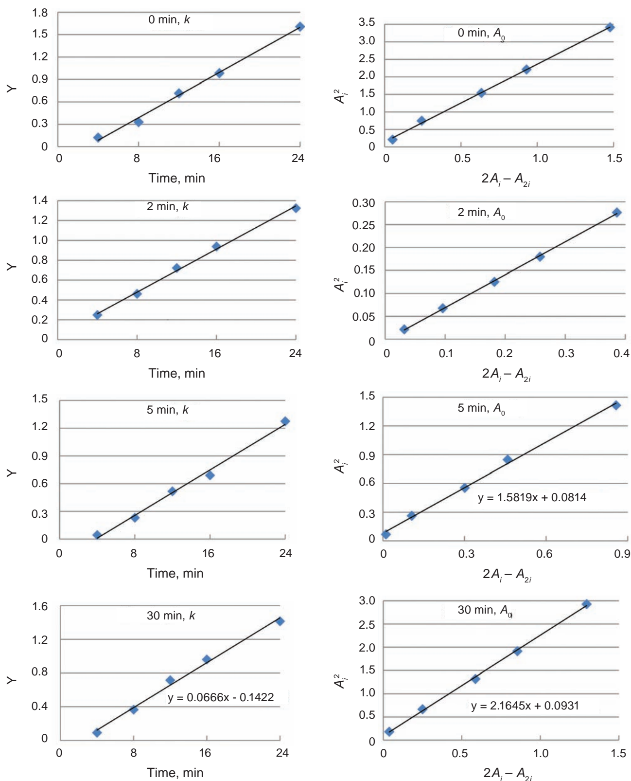
Fig. 6. Calculations of k_i and A_0 from the data on antibody binding kinetics to immobilized antigen presented in Fig. 5, B using linear functions Y = \ln\left(\frac{A_i}{A_{2i} - A_i}\right) vs. t_i and A_i^2 vs. 2A_i - A_{2i} . The linear functions obtained with Microsoft Excel are presented. The tangents of their decays are equal to k_i (on graphs to left) or A_0 (on graphs to right) for antibody samples (0 min as control) or treated 2, 5 or 30 min in 25% TFE at 0°C
