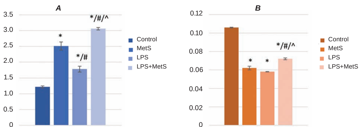
Fig. 2. A – Activity of iNOS in rat biceps femoris, \mu\text{mol}/\text{min} per g of protein; B – Activity of cNOS in rat biceps femoris, \mu\text{mol}/\text{min} per g of protein. *The data are statistically significantly different from the control group ( P < 0.05 ); #the data are statistically significantly different from the experimental metabolic syndrome group ( P < 0.05 ); ^the data are statistically significantly different from the group of stimulation of the organism by bacterial lipopolysaccharide ( P < 0.05 )
