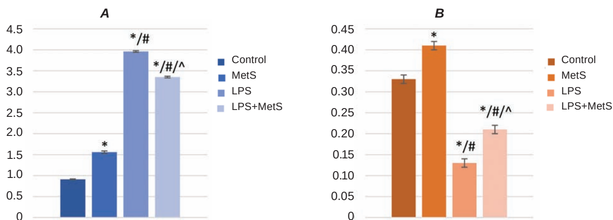
Fig. 5. A – Concentration of \text{ONOO}^- in rat biceps femoris, \mu\text{mol/g} of tissue; B – Concentration of S-nitrosothiols in rat biceps femoris, \mu\text{mol/g} of tissue. *The data are statistically significantly different from the control group ( P < 0.05 ); #the data are statistically significantly different from the experimental metabolic syndrome group ( P < 0.05 ); ^the data are statistically significantly different from the group of stimulation of the organism by bacterial lipopolysaccharide ( P < 0.05 )
