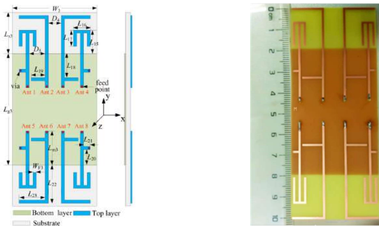
Fig. 7. Geometry and photography of the compact MIMO 8-element antenna [52]
