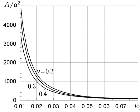
Fig. 2. The dependence of the dimensionless amplitude on dimensionless wave number k_1 at different values of the Poisson coefficient \nu .
