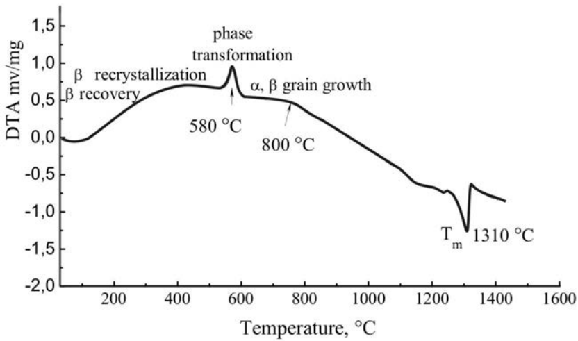
Fig. 2. DTA curve of the 5 h mechanically alloyed AlCuNiFeCr HEA powder.
