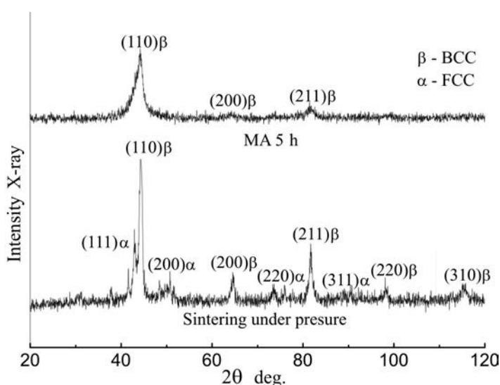
Fig. 4. XRD patterns of equiatomic AlCuNiFeCr HEA after MA and sintering at 800 °C with 5 GPa pressure for 0.5 h.
