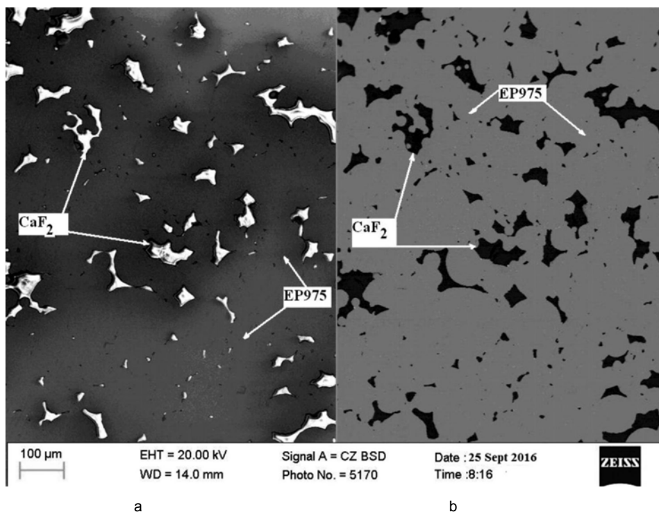
Fig. 1. Microstructure of material EP975 + 6 % \text{CaF}_2 (raster electron microscope). a – image in secondary electrons, b – phase contrast image.
