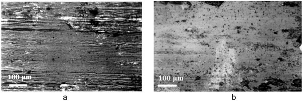
Fig. 2. Images of friction surfaces. a – material EP975 + 6 % CaF 2 , b – counterface of steel R18.
