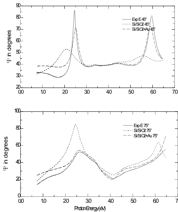
Fig. 6. Experimental spectra of the angle \psi for angles of incidence of 45° and 75° for the sample without annealing (solid) and simulated curves with the best fitting for a bare Si/SiO 2 substrate (dotted) and for Si/SiO 2 substrate with a thin film of gold (dashed).
