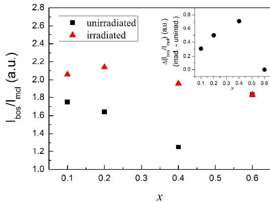
Fig. 5. The ratio of the intensity of the boson peak to the intensity of the main molecular peak at 340\text{ cm}^{-1} , I_{\text{bos}}/I_{\text{mol}} , for unirradiated and \gamma -irradiated glasses of the (\text{As}_2\text{S}_3)_x(\text{GeS}_2)_{1-x} system as a function of composition x . Insert shows the difference, \Delta(I_{\text{bos}}/I_{\text{mol}}) , between values of I_{\text{bos}}/I_{\text{mol}} for \gamma -irradiated (irrad.) and unirradiated (unirrad.) samples.
