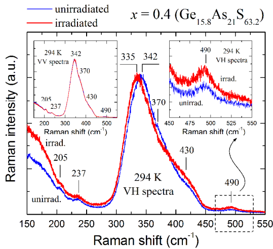
Fig. 1. The normalized VH Raman spectra for unirradiated and \gamma -irradiated glasses of the (\text{As}_2\text{S}_3)_x(\text{GeS}_2)_{1-x} system with x = 0.4 ( \text{Ge}_{15.8}\text{As}_{21}\text{S}_{63.2} ). Inserts show corresponding Raman spectra in VV polarization (left) and VH polarization in the vicinity of 490 \text{ cm}^{-1} band (right).
