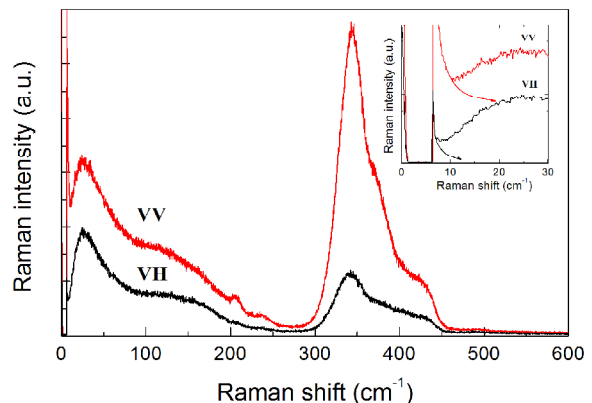
Fig. 4. The polarized-VV and depolarized-VH Raman spectra of (\text{As}_2\text{S}_3)_{0.2}(\text{GeS}_2)_{0.8} glass, taken as an example, with the excess quasi-elastic light scattering in the low-frequency vibrational region well fitted using the Theodorakopoulos-Jäckle model [28] as shown schematically by lines with arrows in insert (see the text for details).
