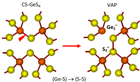
Fig. 7. The schematic illustration of \gamma -induced covalent bond switching heteropolar or heteronuclear Ge – S bonds in the corner-shared (CS) tetrahedral configuration into homopolar or homonuclear S – S bonds [the reaction (2) with the CS- \text{GeS}_4 configuration: (\text{Ge}-\text{S})\rightarrow(\text{S}-\text{S}) ] accompanied by formation of atomic pairs of positively charged over-coordinated sulfur and negatively charged under-coordinated germanium ( \text{S}_3^+ + \text{Ge}_3^- ), VAP defects (see the text for details).
