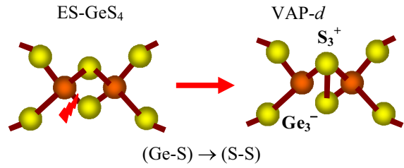
Fig. 8. The schematic illustration of \gamma -induced covalent bond switching heteropolar or heteronuclear Ge – S bonds in the edge-shared (ES) tetrahedral configuration into homopolar or homonuclear S – S bonds [the reaction (3) with the ES- \text{GeS}_4 configuration: (\text{Ge}-\text{S})\rightarrow(\text{S}-\text{S}) ] accompanied by formation of bound atomic pairs of positively charged over-coordinated sulfur and negatively charged under-coordinated germanium defects ( \text{S}_3^+ \cdot \text{Ge}_3^- ), VAP- d defects (see the text for details).
