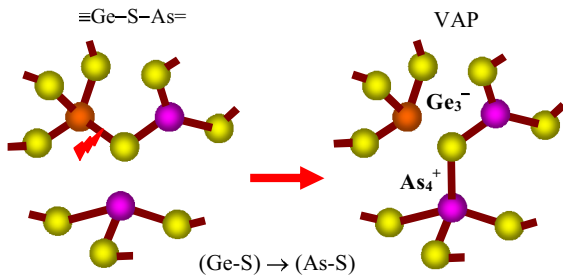
Fig. 6. The schematic illustration of \gamma -induced covalent bond switching heteropolar or heteronuclear Ge – S bonds into heteropolar or heteronuclear As – S bonds [the reaction (1) with the \equiv\text{Ge}-\text{S}-\text{As}=\text{} configuration: (\text{Ge}-\text{S})\rightarrow(\text{As}-\text{S}) ] accompanied by formation of atomic pairs of positively charged over-coordinated arsenic and negatively charged under-coordinated germanium \text{As}_4^+ + \text{Ge}_3^- , VAP defects (see the text for details).
