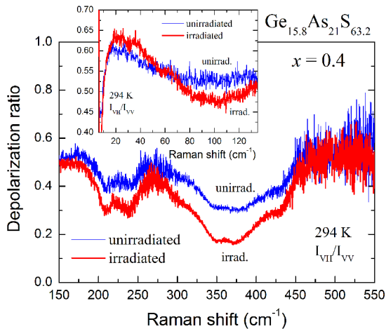
Fig. 2. The high-frequency depolarization ratio spectra ( \rho(\omega) = I_{\text{VH}}/I_{\text{VV}} ) for unirradiated and \gamma -irradiated glasses of the (\text{As}_2\text{S}_3)_x(\text{GeS}_2)_{1-x} system with x = 0.4 ( \text{Ge}_{15.8}\text{As}_{21}\text{S}_{63.2} ). Insert shows respective low-frequency depolarization ratio spectra.
