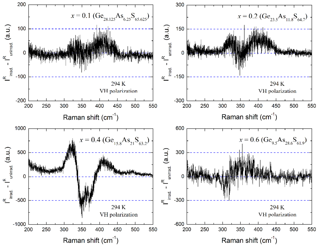
Fig. 3. The differential depolarized Raman spectra between \gamma -irradiated ( I_{\text{irrad.}}^{\text{R}} ) and unirradiated ( I_{\text{unirrad.}}^{\text{R}} ) glasses of (\text{As}_2\text{S}_3)_x(\text{GeS}_2)_{1-x} ( x = 0.1, 0.2, 0.4, 0.6 ) system. All the spectra were normalized to the intensity of the main Raman band at 340 \text{ cm}^{-1} before subtraction.
