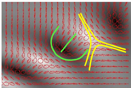
Fig. 5. The polarization distributions against the background of the right hand polarized component: \alpha_0 = 2^\circ , \psi = 210^\circ , w_0 = 5 m, z = 2 cm.
