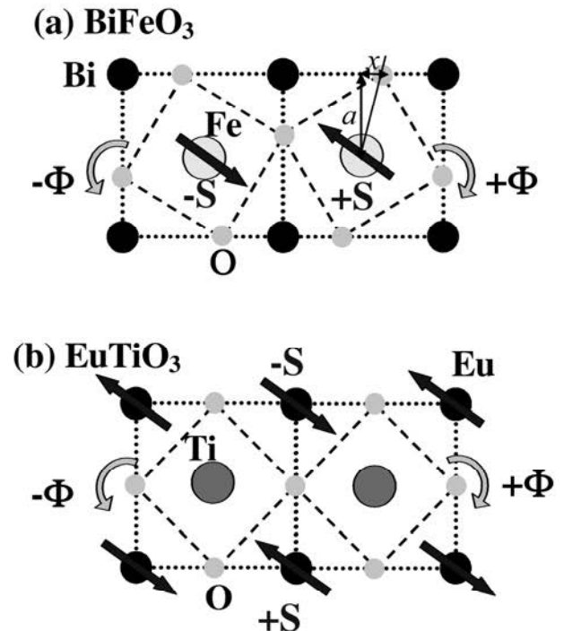
Fig. 2. The structural antiferrodistorsive order parameter is a pseudovector of the angle of rotation of oxygen octahedra in multiferroics \text{BiFeO}_3 (a) and \text{EuTiO}_3 (b). Adapted from Ref. [7]
