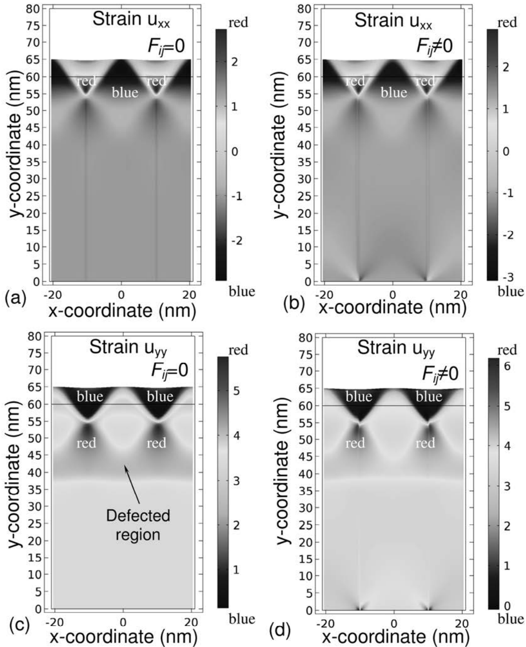
Fig. 11. Maps of spatial distribution of elastic strain components u_{xx} (a, b) and u_{yy} (c, d) in the cross-section of the \text{PbTiO}_3 film at room temperature in the cases when flexoelectric coupling is not included (a, c) and included (b, d) into consideration. N_0 = 2 \cdot 10^{26} \text{ m}^{-3} , other material parameters are listed in Ref. [22]. See colour in electronic version
