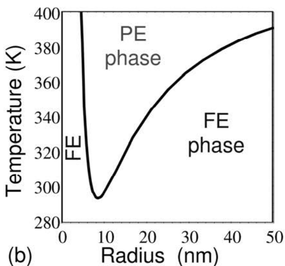
Fig. 4. (a) Dependence of the main components of the biquadratic magnetoelectric coupling tensor (12, 21, 22) on the radius of multiferroic nanoparticle \text{BiFeO}_3 . Adapted from Refs. [5, 10]. (b) Phase diagram of a nanoparticle \text{BaTiO}_3 in the coordinates "temperature-particle radius". PE – non-polar paraelectric phase, FE – polar ferroelectric phase. Adapted from Refs. [5, 11].
