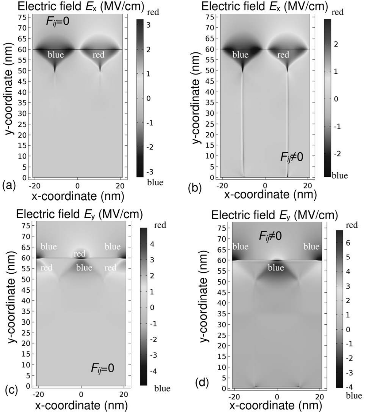
Fig. 9. Maps of spatial distribution of electric field components E_x (a, b) and E_y (c, d) in the cross-section of the \text{PbTiO}_3 film at room temperature in the cases when flexoelectric coupling is not included (a, c) and included (b, d) into consideration. Film thickness h = 60 nm and h_0 = 25 nm (see Fig. 1b). N_0 = 2 \cdot 10^{26} \text{ m}^{-3} , other material parameters are listed in Ref. [22]. See colour in electronic version
