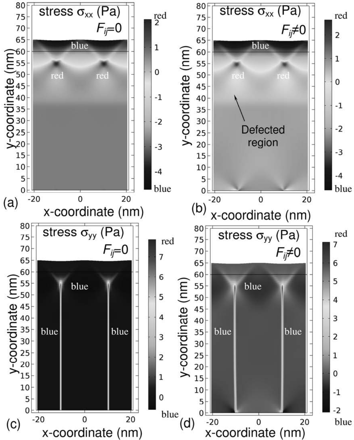
Fig. 10. Maps of spatial distribution of elastic stress components \sigma_{xx} (a, b) and \sigma_{yy} (c, d) in the cross-section of the \text{PbTiO}_3 film at room temperature in the cases when flexoelectric coupling is not included (a, c) and included (b, d) into consideration. N_0 = 2 \cdot 10^{26} \text{ m}^{-3} , other material parameters are listed in Ref. [22]. See colour in electronic version
