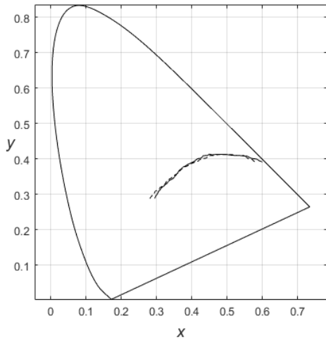
Fig. 4. Results of the black body line simulation (solid line – the resulting functional dependence, dashed – reference data).
