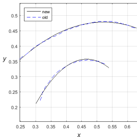
Fig. 3. Lines limiting the scope of the existence of the coordinates for light sources.
