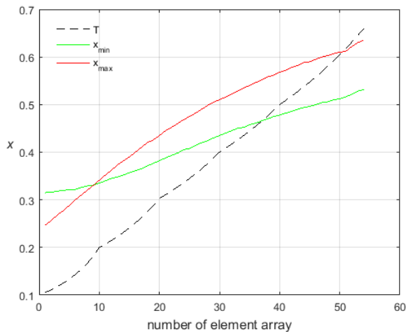
Fig. 2. Relationship between the coordinate values x and T .
