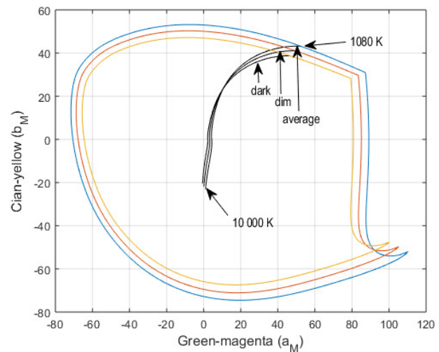
Fig. 7. Changes in the coordinates of the black body line, depending on the conditions of observation.
