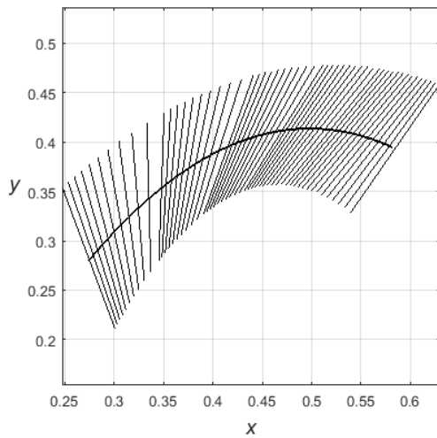
Fig. 5. Isothermal line and line of the black body obtained using the analytical expressions (1)–(7).
