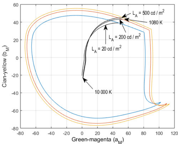
Fig. 6. Changes in the coordinates of the black body line, depending on the adapting luminance ( L_A ).
