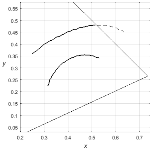
Fig. 1. Area describing the coordinates of the color temperature is constructed using the isothermal lines.
