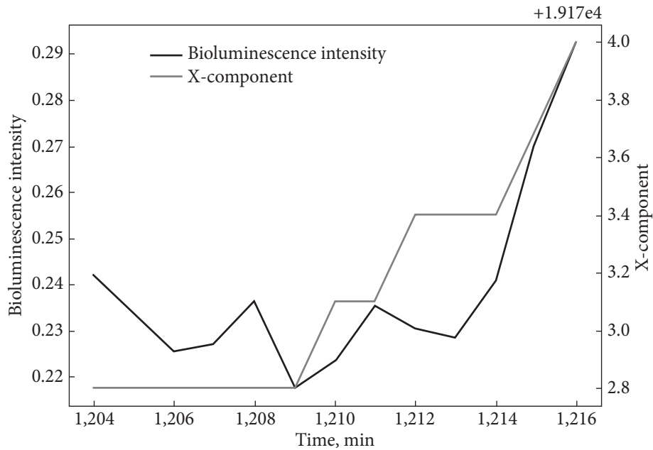
Fig. 3. Changes in the bioluminescence intensity of P. phosphoreum bacteria and X-component within time portion 1204 — 1216 on March 4, 2020. Note: Here and in Figs. 4-6, bioluminescence intensity data are given in conventional units, and the geomagnetic field strength — in nanotesla (nT).
