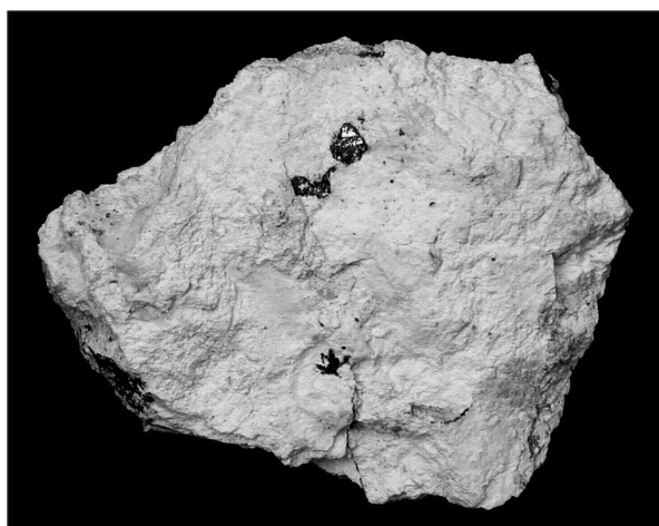
Fig. 4. Layered crystal of telluronevskite in secondary quartzite; size of specimen ~5.5 cm (Poruba pod Vihorlatom)
