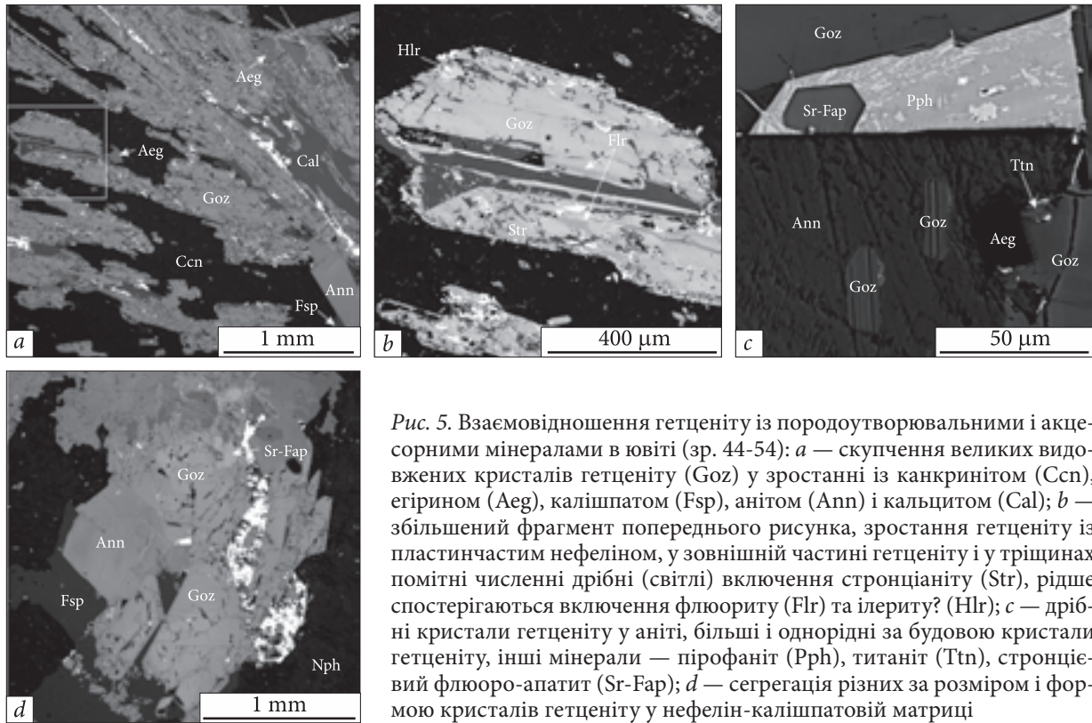
Fig. 5. Relationship of götzenite with rock-forming and accessory minerals of juvite (sample 44-54): a — accumulation of coars elongated grains of götzenite (Goz) in association with cancrinite (Ccn), aegirine (Aeg), feldspar (Fsp), annite (Ann) and calcite (Cal); b — a magnified parth of the previous figure with the intergrowth of götzenite and plates of nepheline. The fine numerous (light) inclusions of strontianite (Str) are widespread in the outer part and in the cracks of the götzenite, less frequent is inclusions of fluorite (Flr) and hilairite? (Hlr); c — a fine zoned (or intergrowth with nepheline?) grains of götzenite in annite and coarse homogeneous grains of götzenite, other minerals — pyrophanite (Pph), titanite (Ttn), strontium fluorapatite (Sr-Fap); d — aggregate of götzenite grains of different sizes and shapes in nepheline-feldspar matrix
