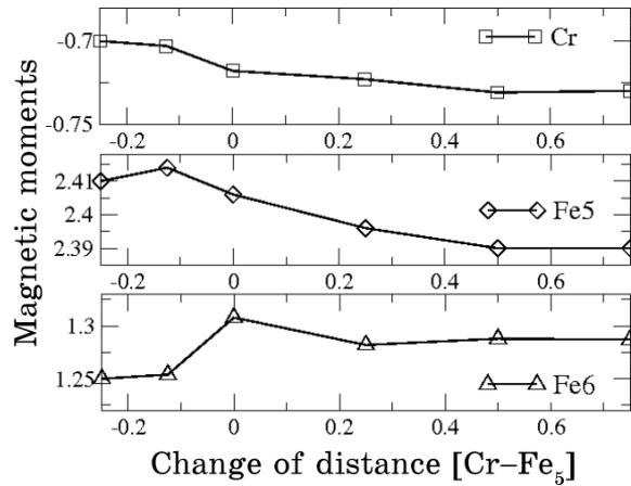
Fig. 3. Local magnetic moments of the atoms in \text{Fe}_5\text{--Cr--Fe}_6 triad versus the displacement \Delta = [\text{Fe}_5\text{--Cr}] - [\text{Fe}_5\text{--Cr}]^0 of Cr along the (100) axis. Here, [\text{Fe}_5\text{--Cr}]^0 is the equilibrium distance between \text{Fe}_6 and Cr.
