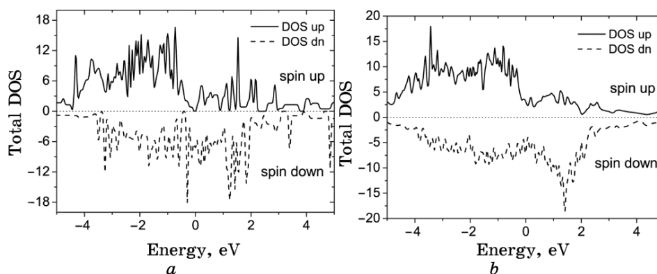
Fig. 6. Total density of states for structures optimized using (a) LDA approach and (b) spin-polarized LSDA approximation. The Fermi level corresponds to E = 0 .
