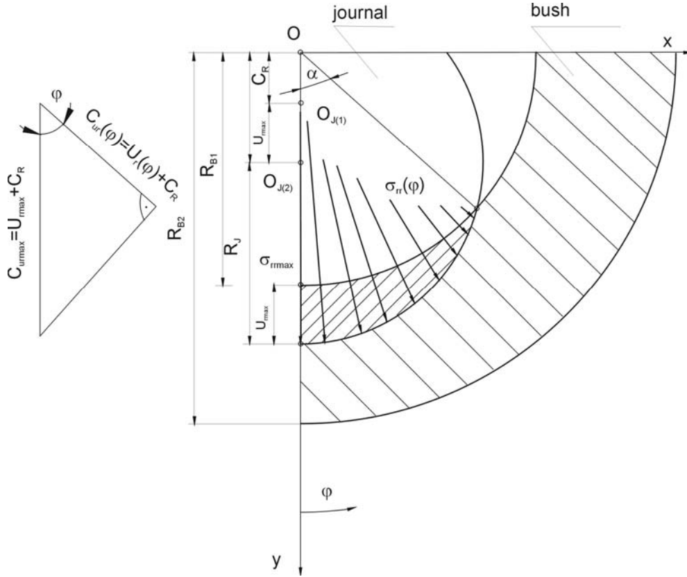
Fig. 2. State of stresses and deformation in the plain journal bearing bush.
