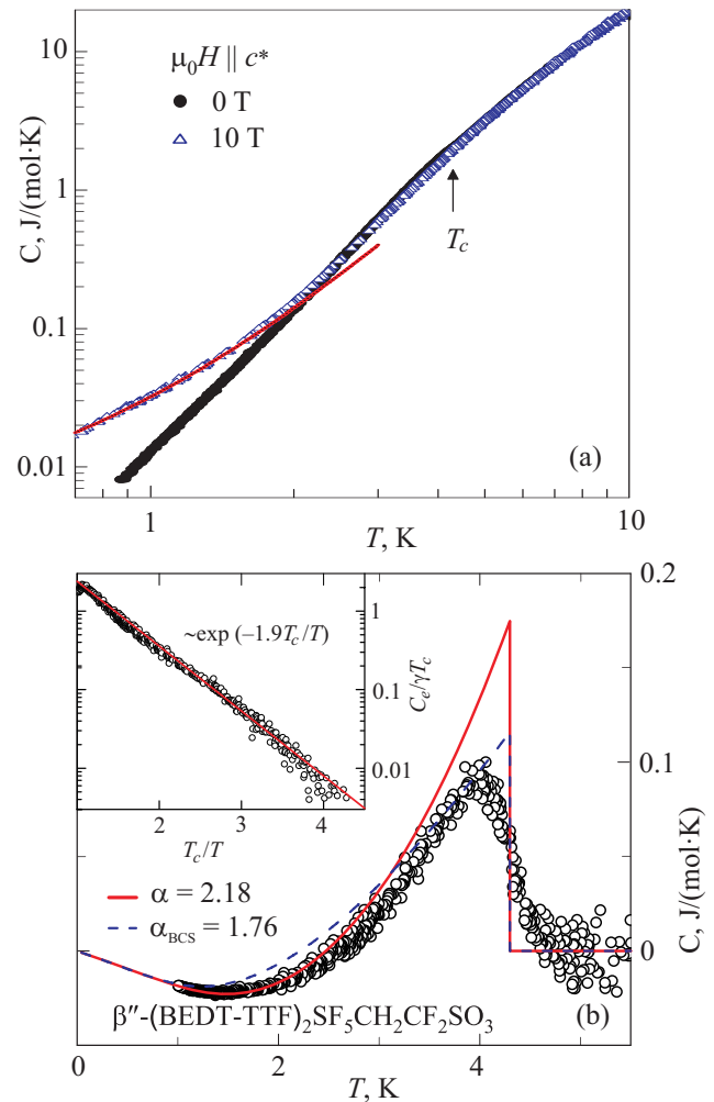
Fig. 5. (a) Temperature dependence of the specific heat of \beta'' -(BEDT-TTF) _2 SF _5 CH _2 CF _2 SO _3 in a double-logarithmic scale. Data in the superconducting state in zero field and in the normal state at 10 T applied perpendicular to the BEDT-TTF planes are shown. The solid line is a fit to the 10-T data below 2 K using a linear and cubic term. (b) Temperature dependence of the specific-heat difference between the superconducting and normal state. The lines show the BCS behavior for weak coupling (dashed) [30] and moderately strong coupling (solid) [31]. The inset shows the electronic part of the specific heat, C_e , divided by \gamma T_c as function of T_c/T . The solid line shows the exponential vanishing of C_e towards low T .
