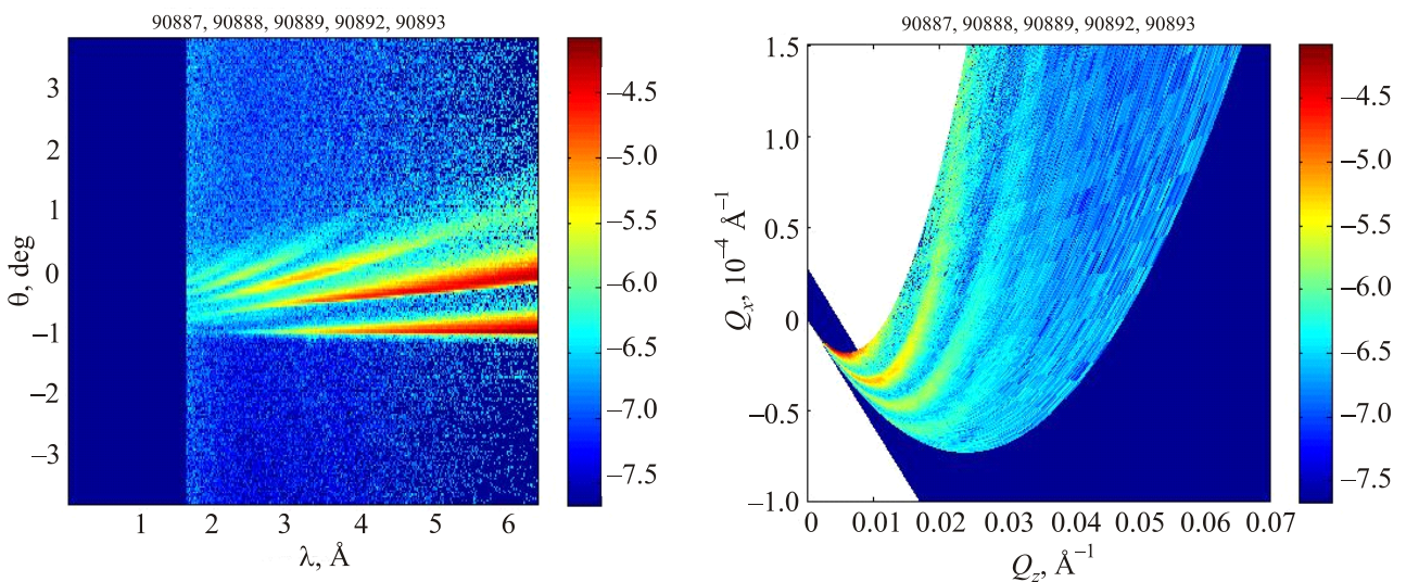
Fig. 4. (Color online) Reflectivity signal maps shown on an area detector from a D_2O surface in a sample cell of 35 mm diameter. The neutron beam's horizontal dimension is comparable with the cell diameter. We can see a periodic pattern in the reflection signal that can be explained by the interference of neutron waves on a curved surface.
