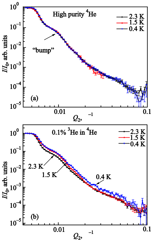
Fig. 1. (Color online) Surface reflectivity curves collected at different temperatures: 2.3, 1.5 and 0.4 K from (a) isotopically purified helium; and (b) 0.1 % ^3\text{He}/^4\text{He} mixture. We hypothesize that the seemingly anomalous “bump” indicated by the arrow in Fig. 1(a) is attributable to optical distortion caused by the liquid helium meniscus.
