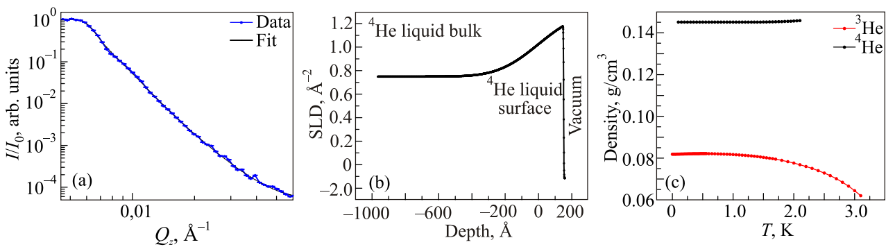
Fig. 2. (Color online) (a) High-purity ^4\text{He} NR curve with fit, taken with a beam footprint 70% the size of the sample can diameter. (b) SLD profile used to generate the NR fit in the first panel. (c) Low-temperature liquid densities for ^3\text{He} and ^4\text{He} isotopes.
