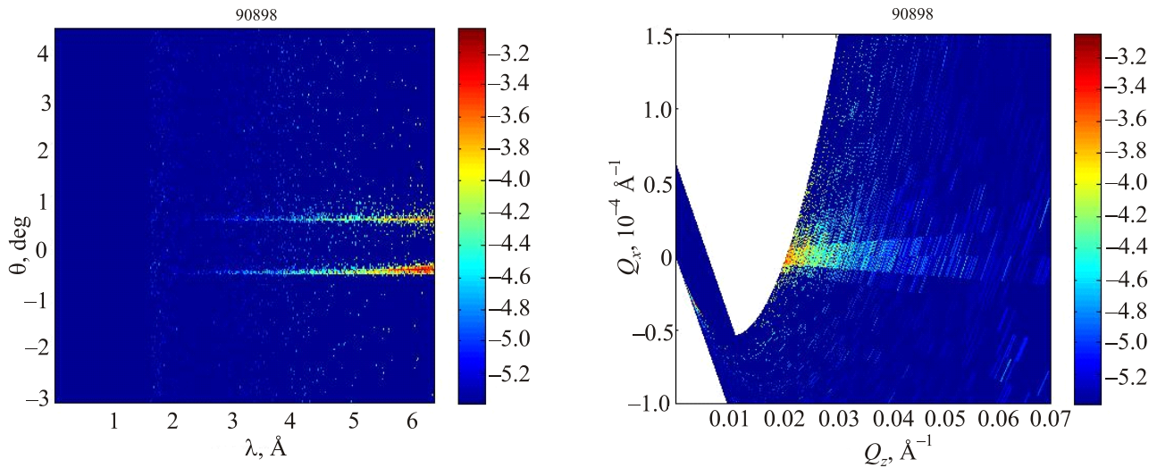
Fig. 3. (Color online) Reflectivity signal maps shown on an area detector from a D_2O surface in a sample cell of 65 mm diameter. The neutron beam's horizontal dimension is significantly smaller than cell's diameter. There is no distortion due to the effect of the meniscus.
