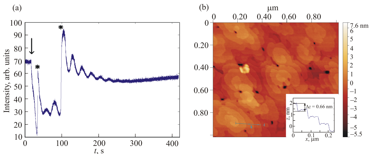
Fig. 1. (Color online) RHEED intensity vs time graph which shows the oscillations of the specular reflected beam for the first few unit cells of the cuprate, after which the amplitude of the oscillation goes to zero, indicating an island-like growth fashion. The arrow indicates the start of the PLD process, while the asterisks show the instances where the electron beam intensity has been increased manually (a). The AFM data shows the screw-island growth mode of a typical cuprate film on LSAT. The step heights coincide with half a unit cell of NC(C)O ( 1.2\text{ nm} ) (b).
