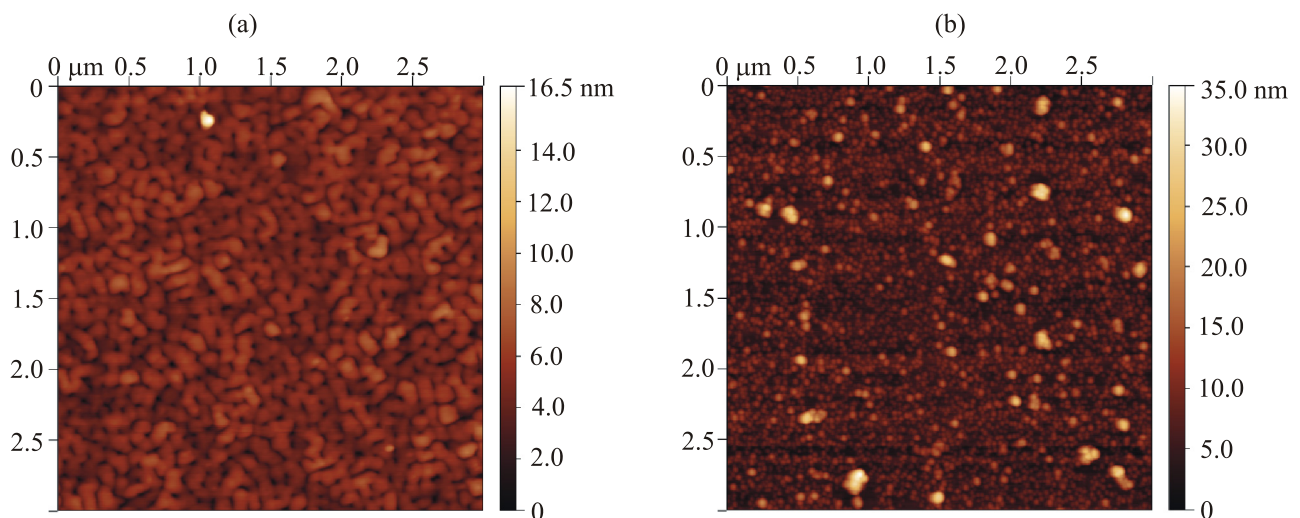
Fig. 4. (Color online) AFM images of the surface of the bilayer before (a) and after (b) IL gating experiments. Before the experiments, the AFM image shows that NCCO has a topography which is island-based. The roughness of the sample is 0.87 \text{ nm} (a). After the experiments, the surface lost the former characteristics, and has a higher roughness of 2.35 \text{ nm} (b).
