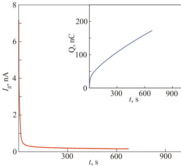
Fig. 5. I_g(t) curve for a V_g of 2.5 V at 210 K. The inset shows the total accumulated charge Q vs time, calculated by integrating I_g(t) . The total accumulated charge Q exceeds the value that one would expect for a purely electrostatic charge of the NCCO layer, i.e. roughly 5 nC.
