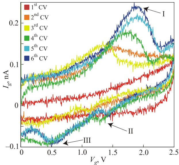
Fig. 3. (Color online) Plots showing 6 CV scans. The first cyclic voltammogram does not show any peaks and indicates a chemically pure IL, while the others show peaks increasing in amplitude as a function of the cycle number. As the number of CV scans increases, several peaks (I, II and III) start to appear. Peak I is located between 1.35 and 1.95 V and indicates an initial reduction. Peak II and III are located between 1.1 and 1.435 V, and 0.29 and 0.55 V, respectively. We observe that the potential separation between peaks I and II is 0.27 \text{ V} < \Delta V < 0.51 \text{ V} . Furthermore, the amplitude of peak I is a factor 3 to 10 higher than that of peaks II and III.
