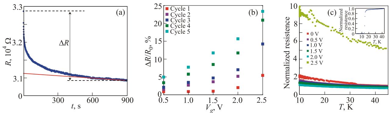
Fig. 6. (Color online) R(t) curve recorded when at t = 0 s a V_g of 0.5 V is applied. The curve shows a change \Delta R , defined as the difference between R at t = 0 s ( R_0 ) and the value of the tangent line at t = 0 s of R at t = 900 s (a). The observed relative change in R as a function of gate voltage and cycle number at 210 K. The change in R is systematic and becomes larger as V_g and the number of cycles increases (b). Normalized resistance of the NCCO/NCO channel plotted as a function of T for V_g = 0 V, +0.5 V, +1.0 V, +1.5 V, +2.0 V and +2.5 V. The behavior is semiconductor-like, and shows a systematic decrease of the resistance up to a gate voltage of +2.0 V. However, applying a gate voltage of +2.5 V leads to sample degradation. The inset figure shows the same type of graph for a film of similar doping which has not been IL gated, showing a critical temperature onset of 12 K (c).
