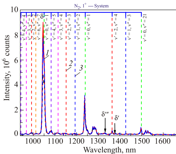
Fig. 5. (Color online) Comparison of the spectra in the range 900–1650 nm observed with the Avantes spectrometer during the injection of nitrogen-helium gas mixture N 2 :He = 1:100 (solid line) and 1:200 (dashed line) into a rotating beaker with He II for different rotational speeds: 3 rad/s (black, 1), 4 rad/s (red, 2), 7.5 rad/s (blue, 3).
