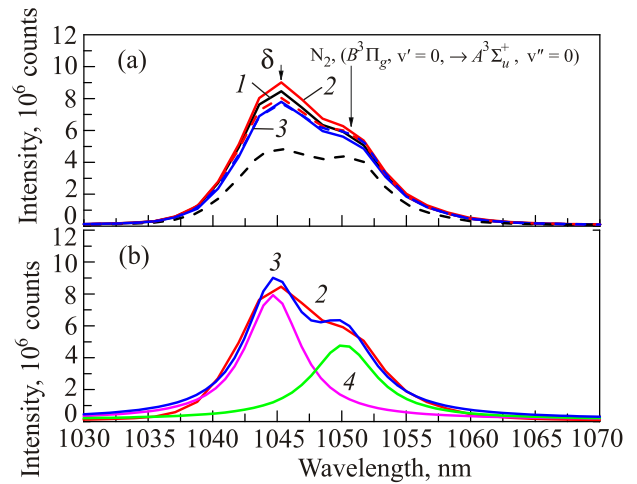
Fig. 6. (Color online) (a) Comparison of the spectra of overlapping N atom \delta -group and N 2 ( B^3\Pi_g, v'=0 \rightarrow A^3\Sigma_u^+, v''=0 ) emissions observed during the injection of nitrogen-helium gas mixtures N 2 :He = 1:100 (solid lines) and 1:200 (dashed lines) into rotating He II for different rotational speeds: 3 rad/s (black, 1), 4 rad/s (red, 2), 7.5 rad/s (blue, 3). (b) Deconvolution of the overlapping spectra of \delta -group and N 2 ( B^3\Pi_g, v'=0 \rightarrow A^3\Sigma_u^+, v''=0 ) emissions. Experimental spectrum of these two bands recorded during injection of N 2 :He = 1:100 gas mixture into beaker rotating at 4 rad/s (red, 2), Lorentzian fitting line for \delta -group emission (magenta, 4), Lorentzian fitting line for N 2 ( B^3\Pi_g, v'=0 \rightarrow A^3\Sigma_u^+, v''=0 ) emission (green, 4), the sum of the fitting lines (blue, 3).
