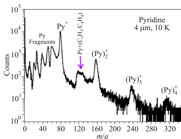
Fig. 4. TOF-SIMS mass spectrum of pyridine condensed at 10 K under impact of the 90 keV \text{O}^{6+} projectiles. Py is observed at m_{\text{Py}} = 79 u. At masses m < m_{\text{Py}} , Py fragments, and at masses m > m_{\text{Py}} , clusters of pyridine (\text{Py})_n with n up to 4 are visible.
