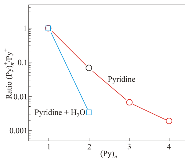
Fig. 5. Relative cluster yields Y(n) of pure Py and a Py– \text{H}_2\text{O} mixture (as indicated), normalized to that of pure pyridine, Y(1) = 1 , as a function of cluster size n .
