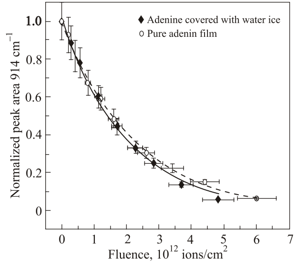
Fig. 2. Evolution area of one of the IR absorption peaks of adenine (914 cm -1 ) with projectile fluence F for pure adenine, and adenine covered with a water layer (as indicated, from [44]).
