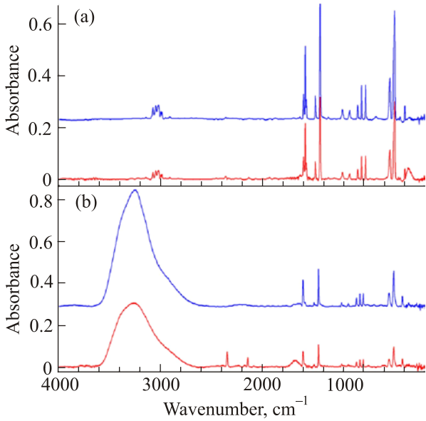
Fig. 1. FTIR spectra obtained by irradiation of (a) pyridine (Py) and of a (b) Py-H 2 O mixture before and after irradiation with O 6+ (90 keV) at 15 K during 50 min. The range of 90 keV oxygen projectiles is about 0.4 μm, the thickness of the deposited layers of the order of 1 μm. The final projectile fluence amounts to 10 15 cm -2 . Spectra “before irradiation” were slightly shifted on the absorbance axis for better visibility.
