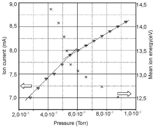
Fig. 5. Ion current inside an ICP near the grid electrode and the mean \text{Ar}^+ ion energy as functions of pressure.
