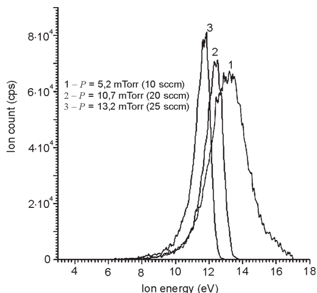
Fig. 2. IEDs of an \text{Ar}^+ ion beam for different pressures without voltage on the acceleration grid. The output power is P = 200 W.
