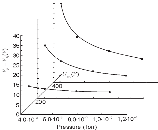
Fig. 6. V_p - V_{1g} as a function of pressure and accelerating voltage.
