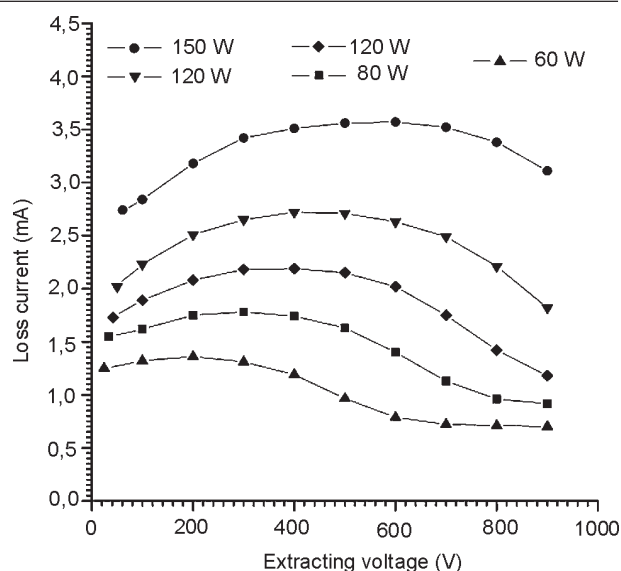
Fig. 4. Loss current due to plasma boundary movement during extraction voltage increase.
