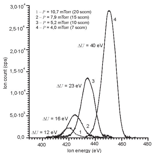
Fig. 3. IEDs of \text{Ar}^+ ions for 4 \cdot 10^{-3} (the highest peak), 5,2 \cdot 10^{-3} ; 7,9 \cdot 10^{-3} and 1,07 \cdot 10^{-2} Torr. The accelerating voltage is 410 V, and the output power is P = 200 W.
