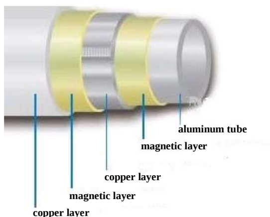
Figure 3 – Protective multi-layer screen
