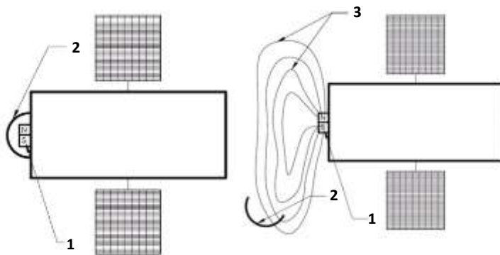
Figure 4 – Principle scheme of devices with permanent magnets, where 1 – permanent magnet, 2 – special protective screen, 3 – generated magnetic field.
