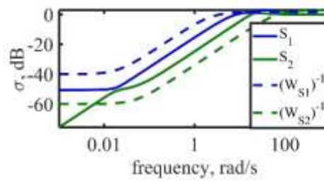
Fig. 7 – Variation of sensitivity function (1-st iteration)
