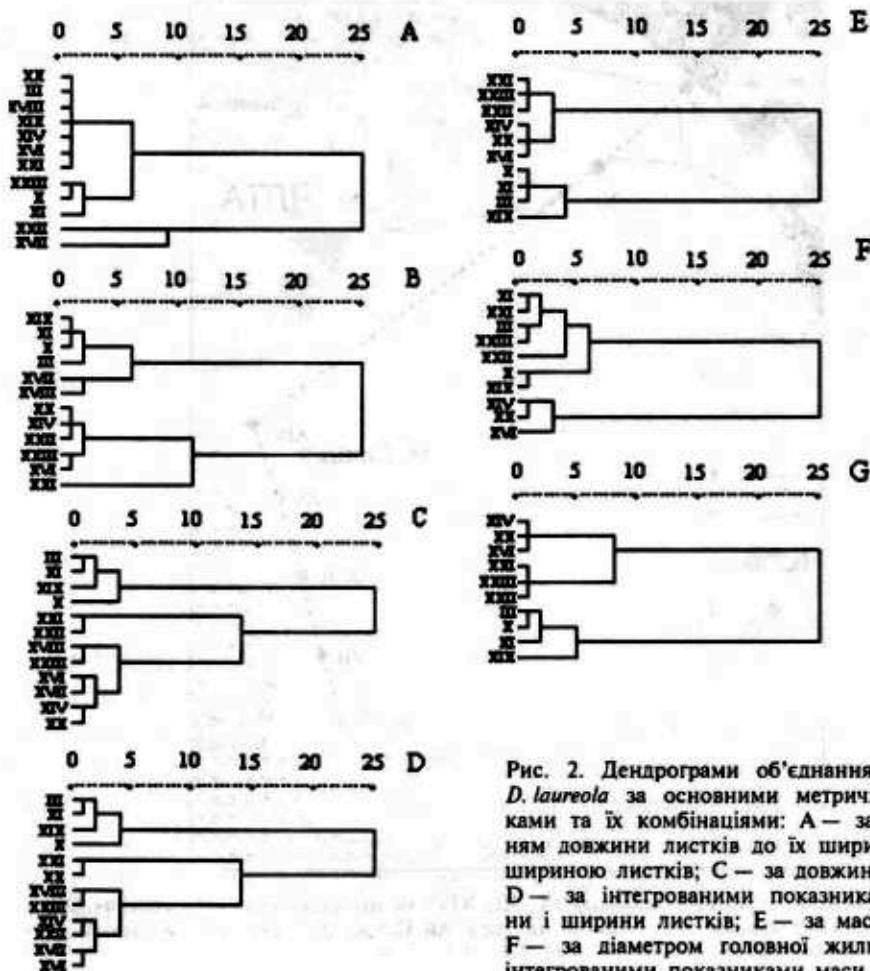
Fig. 2. Dendrograms of the join D. laureola populations by the main metric attributes and its combinations: A — on a ratio are long of leaves to their width; B — on a width of leaves; C — on a long of leaves; D — on a integration parameters the width and long of leaves; E — on a weight of leaves; F — on a diameter of main rib; G — on a integration parameters the weight and diameter of main rib
