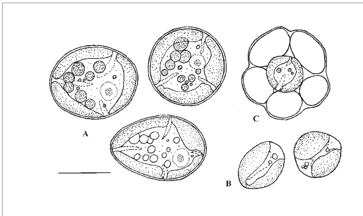
Fig. 11. Leptochlorella arboricola Mikhailyuk sp. nov. A: mature vegetative cells; B: young cells; C: sporangium. Scale bar: 10 \mu m
