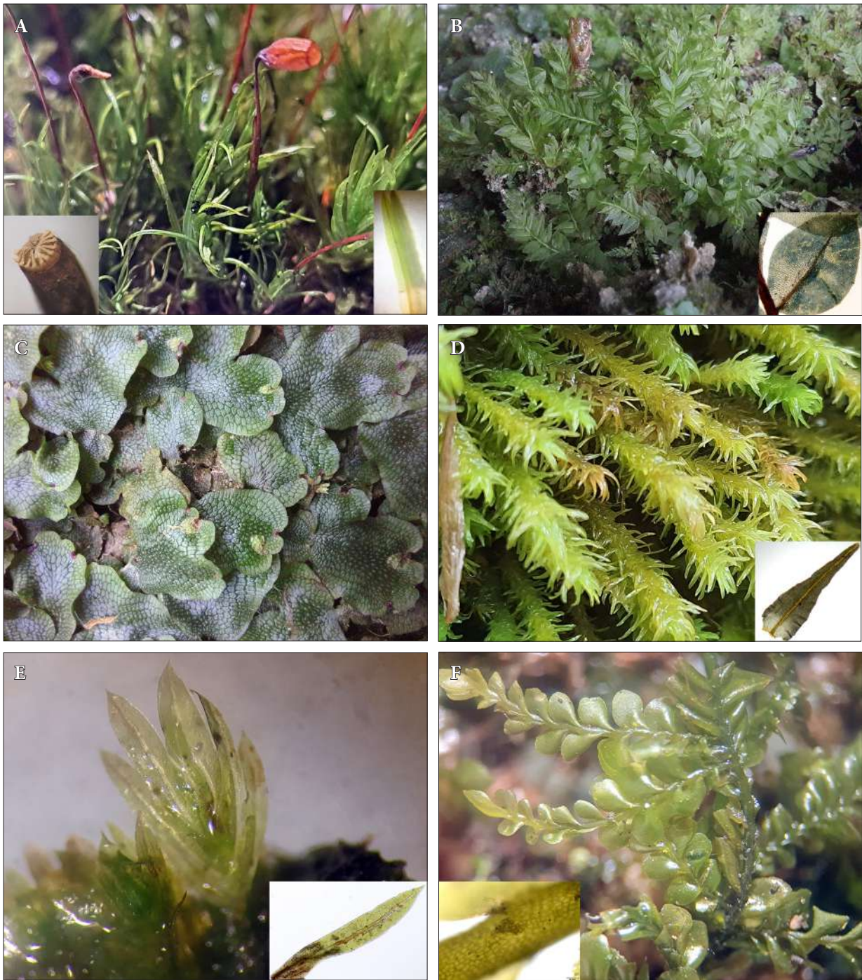
Fig. 5. Bryophytes of the Dumka Cave complex. A: Timmia bavarica ; B: Mnium stellare ; C: Conocephalum salebrosum ; D: Anomodon viticulosus ; E: Fissidens gracilifolius ; F: Pedinophyllum interruptum
