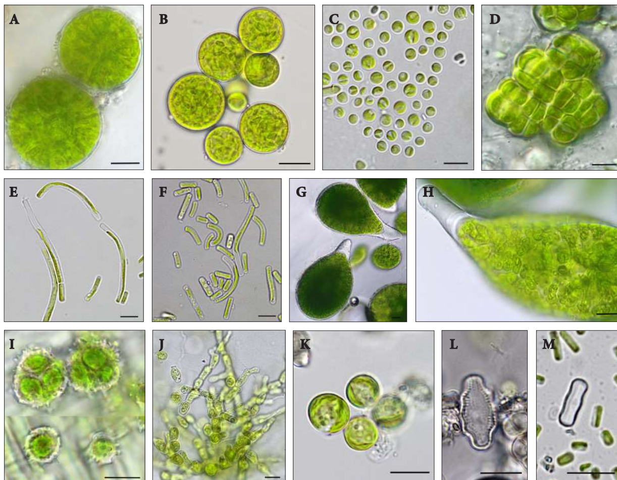
Fig. 3. Eukariotic algae of the Dumka Cave complex. A: Macrochloris dissecta ; B: Bracteacoccus cf. minor ; C: Nannochloris sp.; D: Desmococcus olivaceus ; E, F: Pseudostichococcus undulatus ; G, H: Scotinosphaera sp.; I: Trichiscia granulata (sporangia on top and vegetative cells on bottom); J: Pseudendoclonium cf. arthopyreniae ; K: Coccomyxa cf. viridis ; L: Luticola nivalis ; M: Humidiphila sp. Scale bars: 10 µm
