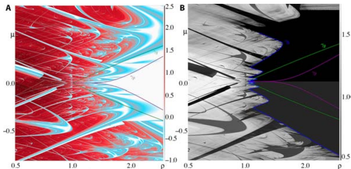
Fig. 12. (A) Chaos and stability windows (“shrims”) in a 4000 \times 4000 -pixel scan of the (\rho, \mu) -parameter plane of the one-dimensional saddle-focus map with \omega = 5 . The heatmap represents the magnitudes (color bar on the right) of Lyapunov exponents computed over trajectories of length 5000 with the red color indicating chaos and the blue/white colors signifying stability. Discontinuities in the color grading correspond to branch-switching in areas of multistability, mostly well-organized for \rho > 1 . (B) 4000 \times 4000 -pixel bifurcation diagram of the map viewed through the lens of Lempel–Ziv complexities of the symbolic binary sequences of long orbits beginning with the same initial point x_1 = \mu : lighter shades signify higher symbolic complexity (color bar on the right). The overlaid curves \gamma_b , \gamma_g , and \gamma_p are the same as in Fig. 11. Despite unbounded and Lyapunov-positive trajectories in much of the \rho > 1 half plane, the symbolic representations of these orbits are very simple for small enough |\mu| , undisturbed by distant homoclinic structures. The shrimp structures from panel (A) appear as windows of relatively lower complexity.
