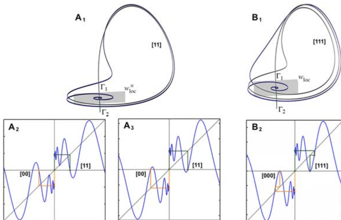
Fig. 6. Comparison of one-sided secondary and tertiary homoclinic orbits. ( A_1 ) A secondary (one-sided) homoclinic orbit (coded as [11] ) to the Shilnikov saddle-focus ( \rho < 1 ) with its two variants in the one-dimensional return maps ( A_2 and A_3 ) ending at different zeros. ( B_1 ) A tertiary (one-sided) homoclinic orbit coded as [111] and its representation in the one-dimensional return map ( B_2 ) where the right forward iterates of the origin attain a critical point touching the horizontal axis — the so-called homoclinic tangency.
