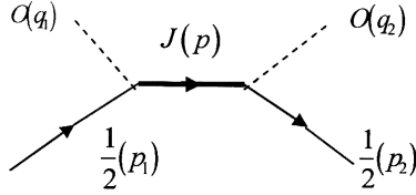
Fig. 1. Feynman diagram for the contributions of higher-spin fermion resonances N^*(J) to the \pi N -scattering amplitudes
