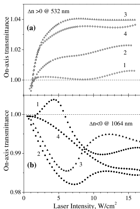
Fig. 4. Normalized on-axis transmittance in the far field versus the laser intensity at 532 (a) and 1064 (b) nm for the crystals cut from the prismatic growth sector: Pr (1), Pr-5 (2), Pr-4 (3) and Pr-3 (4). The sample notation is presented in Table
