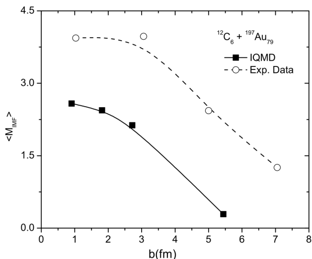
Fig. 4. Mean multiplicity of IMFs vs the impact parameter b , for the experimental data and the IQMD calculations for C + Au at 600 MeV/nucleon
