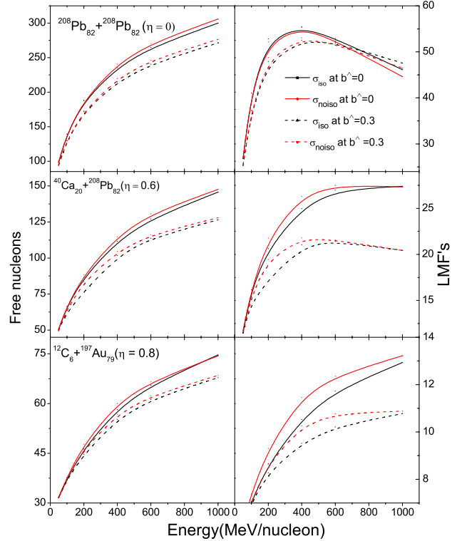
Fig. 1. Multiplicity of free nucleons and LMFs as a function of the energy
