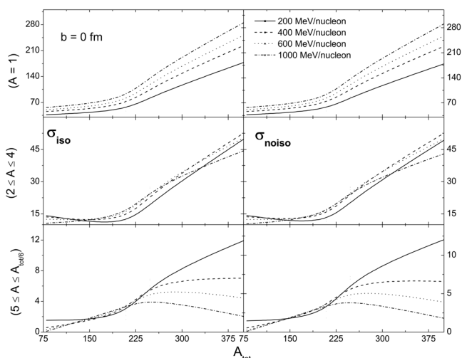
Fig. 3. (Color online) Multiplicity of various fragments vs the total mass of the system ( A_{tot} ) at various energies
