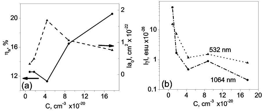
Fig. 4. The concentration dependences of the charge separation efficiency \eta_a , polarizability of photoinduced Ti^{3+} centers a_0 (a), and third hyperpolarizability of a nanoparticle \gamma for picosecond pulsed excitations at 1064 nm and 532 nm (b)
