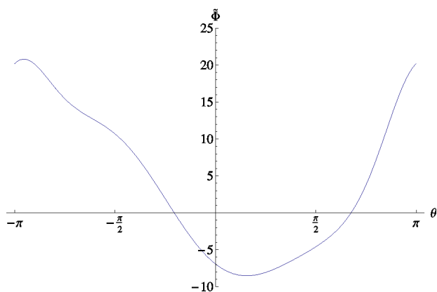
Fig. 10. Dependence of the interaction energy on the angle \theta at r_{\text{OO}} = 2.9757 \text{ \AA}
