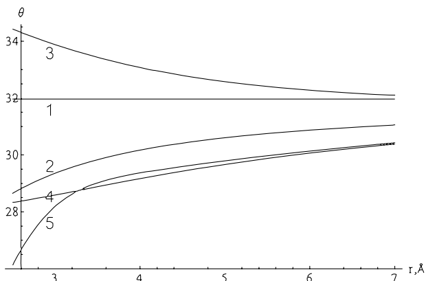
Fig. 6. Radial dependence of the angle \theta_m (5). Angles \alpha , \beta , and \chi remain fixed and correspond to the absolute minimum configuration. Curves 1 – 4 describe the dependence of \theta_m in DD , DQ , QQ , and DO approximations, respectively
