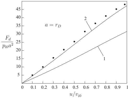
Fig. 4. Velocity dependence of the ion drag force for a = r_D . Symbols \bullet show the present results. Solid line (1) shows the results obtained by the conventional binary collision approach [see Eqs. (28), (29) and (30)]. Solid line (2) shows the results obtained by the modified binary collision approach [see Eqs. (33), (29), and (34)]
