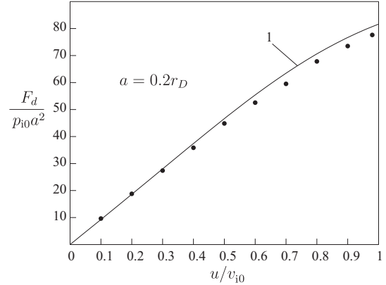
Fig. 2. Velocity dependence of the ion drag force for a = 0.2r_D . Symbols ● show the present results. Solid line (1) shows the results obtained by the conventional binary collisional approach [see Eqs. (28), (29), and (30)]
