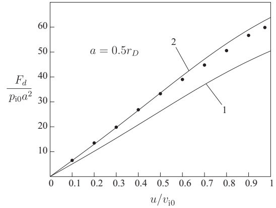
Fig. 3. Velocity dependence of the ion drag force for a = 0.5r_D . Symbols ● show the present results. Solid line (1) shows the results obtained by the conventional binary collisional approach [see Eqs. (28), (29), and (30)]. Solid line (2) shows the results obtained by the modified binary collisional approach [see Eqs. (33), (29), and (34)]
