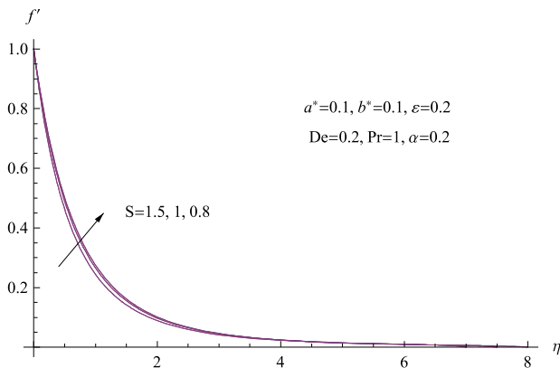
Fig. 3. Behavior of the velocity distribution for various values of S
