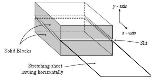
Fig. 1. Schematic of extrusion processes [28]
