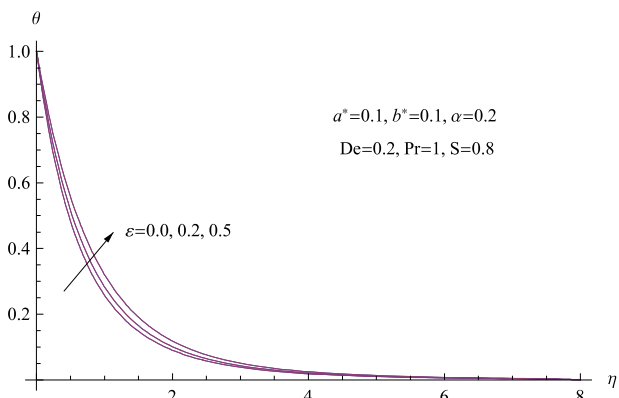
Fig. 10. Behavior of the temperature distribution for various values of \epsilon
