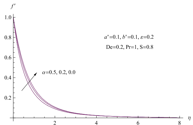
Fig. 8. Behavior of the velocity distribution for various values of \alpha
