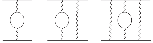
Photons exchange diagrams of eVP contributions
