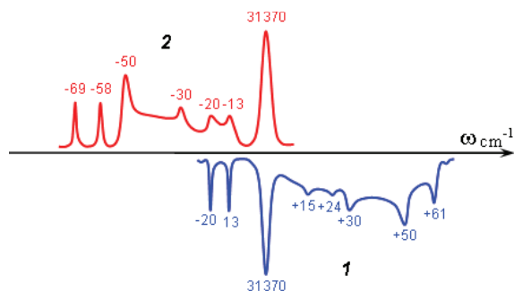
Fig. 3. Schematic representation of the fluorescence (2) and absorption (1) spectra of \alpha -naphthalene fluorine in naphthalene in the impurity band with \nu_{02} = 31370 \text{ cm}^{-1}
