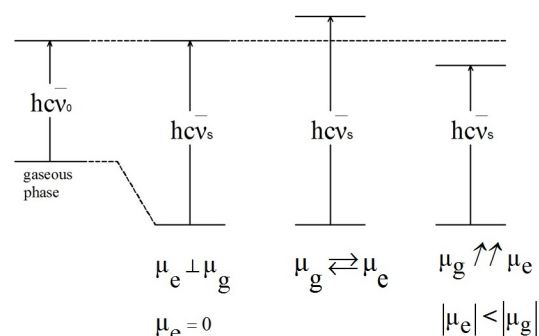
Fig. 4. Spectral shifts determined by the changes in the magnitude and the orientation of dipole moments in the ground and excited states of a spectrally active molecule
