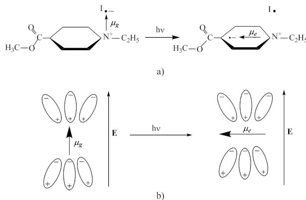
Fig. 1. Chemical structure and the intermolecular charge transfer mechanism in ECMPI complex ( a ); Solvent arrangement in the first solvation shell of complex ECMPI ( b )
