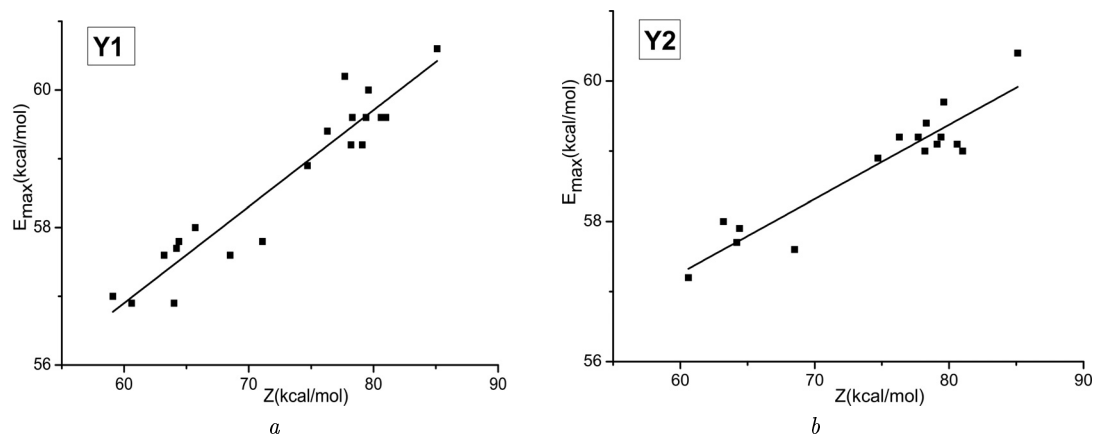
Fig. 5. E_{\max} (kcal/mol) vs. Z (kcal/mol) for: a) Y_1 and b) Y_2 in binary solutions
