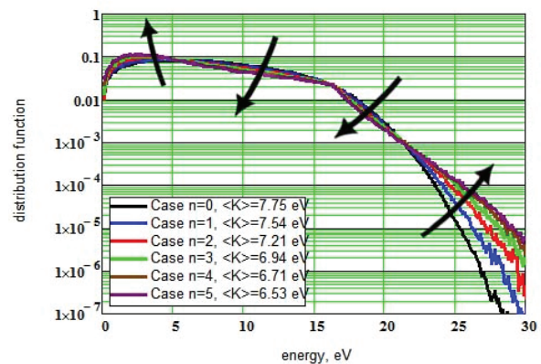
Fig. 3. Electron energy distribution in the drift in the periodic electric field ( E/N = 10 Td, neon, the field period is equal to 4 cm, field intensity – 4 V/cm). Different curves correspond to different values of the exponent field inhomogeneity. The arrows indicate the direction of changes with the increase of fluctuations of the field
