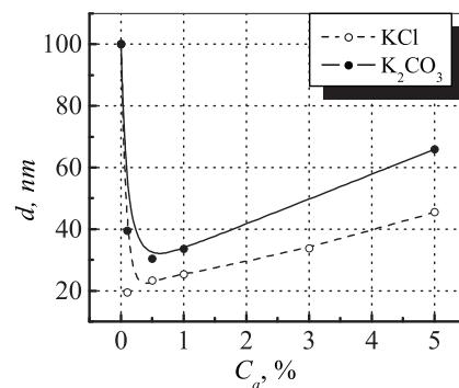
Fig. 3. Size of \text{Al}_2\text{O}_3 particles vs. the additive concentration in the initial fuel (points – experiment; dashed line is an approximation)
