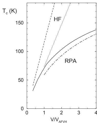
Fig. 6. Influence of dilute impurities on T_c : solid line is the result of pure RPA calculations, dot-dashed line is obtained in the “dirty” RPA; dashed line is the pure HF approximation, dotted line is the “dirty” HF case. Strong coupling calculation is much less affected by the impurities than the HF approximation
