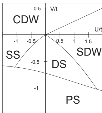
Fig. 1. Mean-field phase diagram of the t - U - V model at half-filling [5]. DS, SS, PS, CDW, and SDW denote d -wave SC, s -wave SC, phase separation, charge-density-wave, and spin-density-wave order, respectively
