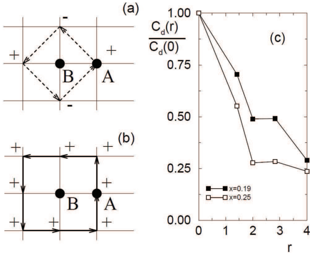
Fig. 3. Two fermions in the large |V| limit of Eq. (1) showing the d_{x^2-y^2} -wave character of the bound state (a); two fermions in the large |V| limit of the t-U-V model (b). The bound state is the s -wave; (c) d_{x^2-y^2} pairing correlations vs the distance r for Eq. (1) at T = 0 studied with the exact diagonalization techniques on a 32-site cluster. The couplings are |V|/t_{11} = 1.0 , t_{20}/t_{11} = 0.4 , and x is indicated. Correlations in the s - and p -channels are negligible [14]
