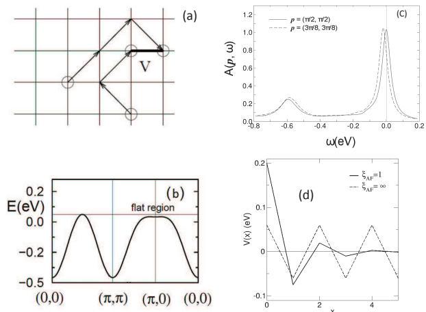
Fig. 2. (a) Schematic representation of model (1). Fermions move within the same sublattice, and interact at distance one; (b) the quasiparticle energy vs the momentum obtained at the half-filling with the use of the t - t' - J model [16]. The result shown is a good fit of Monte Carlo data on a 12 \times 12 cluster at J/t = 0.4 ; (c) Spectral weight A(\mathbf{p}, \omega) for one hole in an antiferromagnet calculated using the rainbow approximation. The first excited state is the ‘‘string state’’ and is located at \omega \sim -0.6 eV; (d) V(x) along the x -axis after the Fourier transformation of the smeared potential V(\mathbf{p}) = \delta(\mathbf{p} - \mathbf{Q}) (see the text); \xi_{\text{AF}} is given in lattice units
