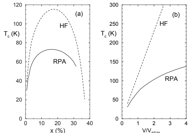
Fig. 4. (a) Critical temperature T_c of model (1) vs the fermionic density x , using t_{11} = 0.165 eV, t_{20} = 0.0435 eV, and V = -0.075 eV, as suggested by the high- T_c phenomenology [9]. The solid line corresponds to the self-consistent RPA approximation. The dashed line is the MF or HF result [9]; (b) T_c vs the coupling constant V , with t_{11}, t_{20} fixed as in (a), at the density where T_c is maximum in (a). V is in units of V_{\text{AFVH}} = -0.075 eV, the coupling used in [9]
