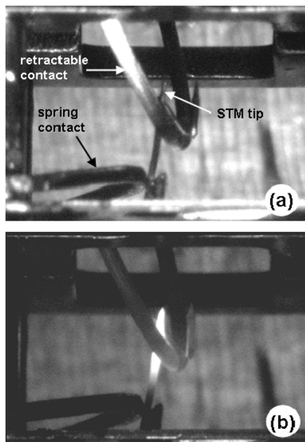
Fig. 1. CCD camera photographs showing (a) actual configuration of the developed tip annealing setup; (b) the same snapshot during the tip annealing at a temperature of 950 K. (Image (b) was acquired with minimal external illumination to take advantage of the CCD camera's near-infrared sensitivity) [6]
