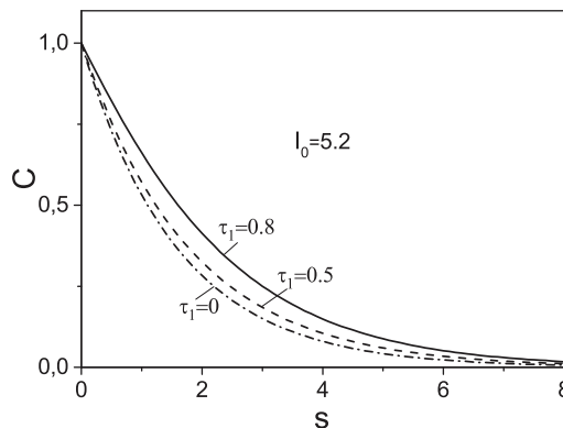
Fig. 10. Correlation functions for the various values of noise p(t) correlations times \tau_1 for the process being before the threshold) with the parameters D = 0.5 , Q = 0.1 , \lambda = 0.5 , \tau_2 = \tau_0 = 0.01
