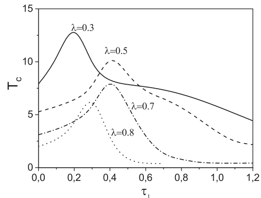
Fig. 5. Dependence of T_C on the self-correlation time \tau_1 of p(t) noise close to the transition point ( I_0 = 5.7 ) for the various cross-correlation strengths \lambda and with the parameters D = 1 , Q = 0.1 , \tau_1 = \tau_2 = \tau_0 = 0.1
